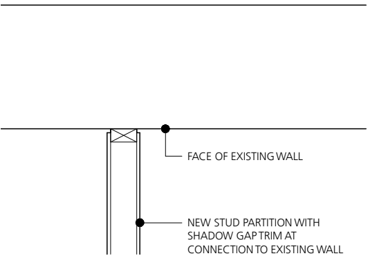
DETAIL P 14
