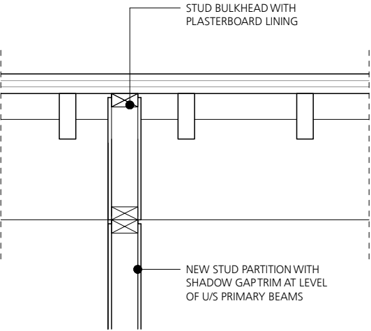
DETAIL P 12
