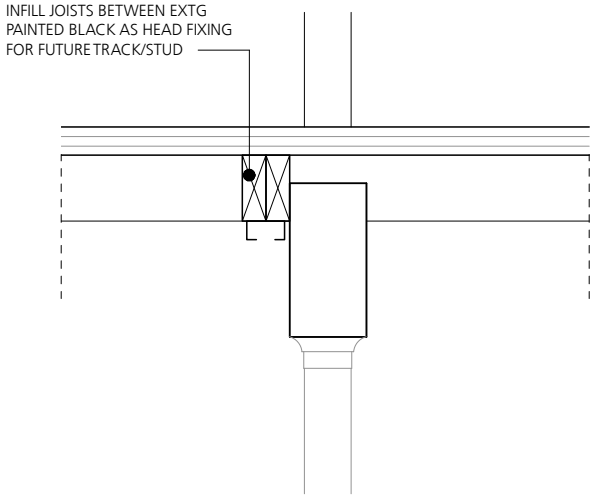
DETAIL P 8
