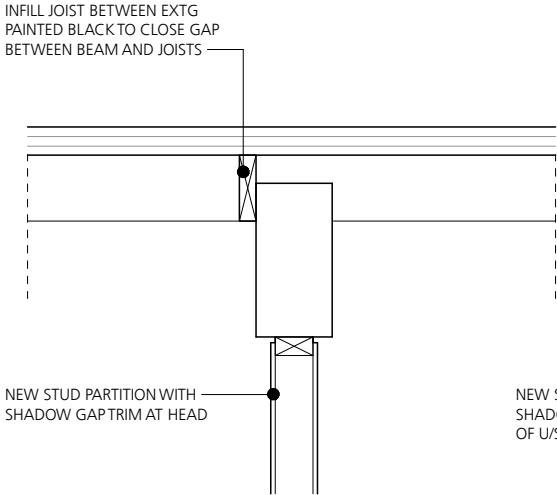
DETAIL P 9
