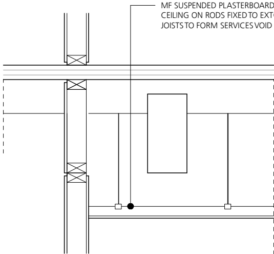
DETAIL P 11
