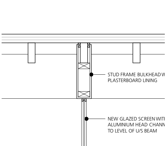
GLAZED SCREEN
