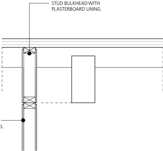
DETAIL P 10
