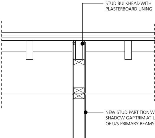
DETAIL P 13
