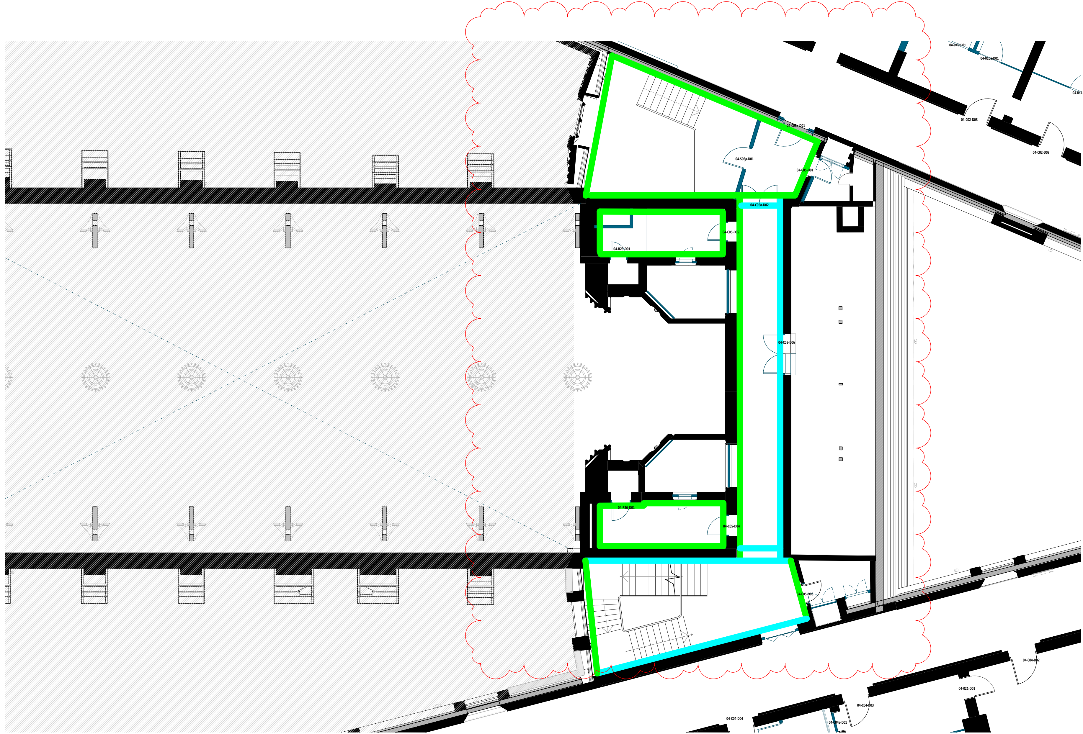
GA PLAN PROPOSED LEVEL 04 - Plaster Removal Plan - 0562 1 : 100
