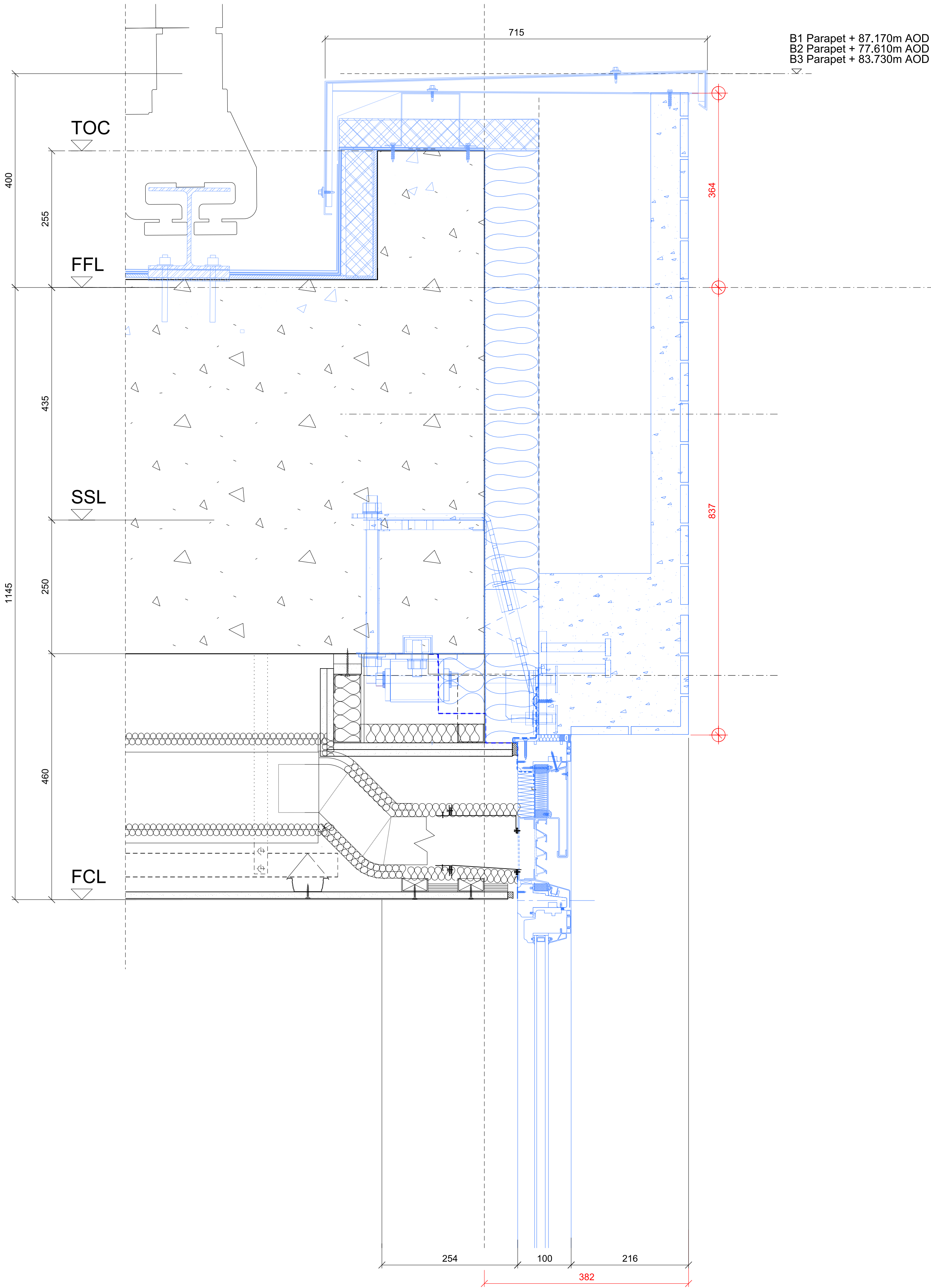
01 Roof Parapet Interface - Active Ventilation Slot 1:5
