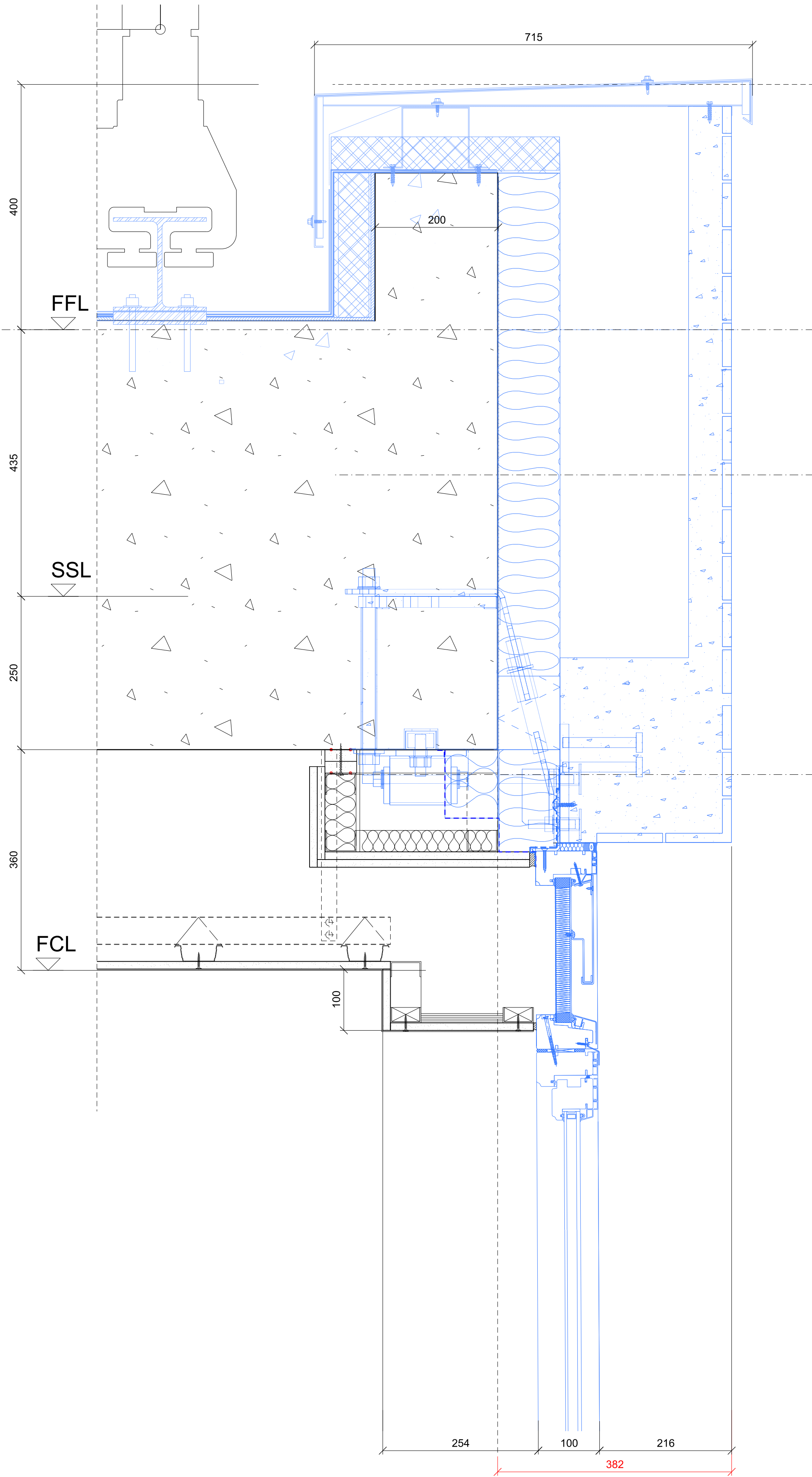
02 Roof Parapet Interface - Insulated Infill Slot 1:5
