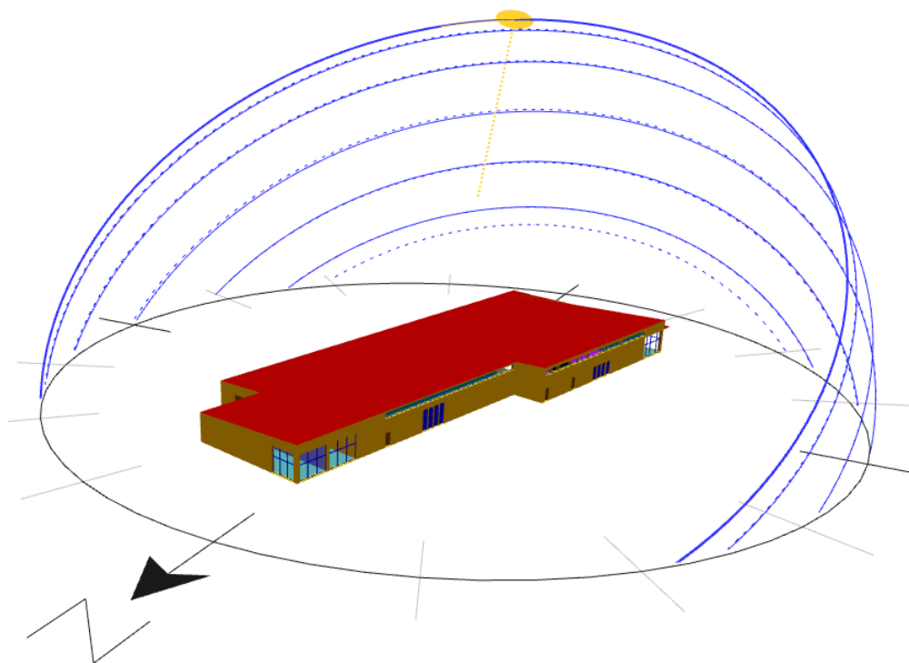
Figure 8 - Orientation & Sun Path Image
