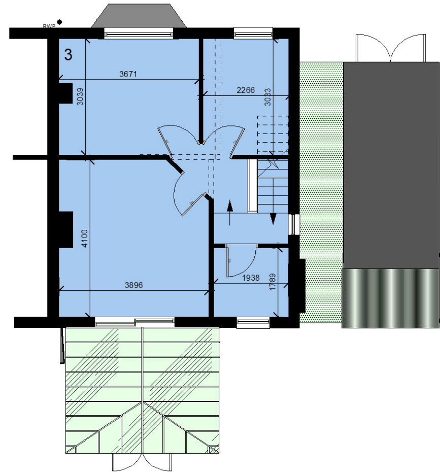
FIRST FLOOR - AS EXISTING
