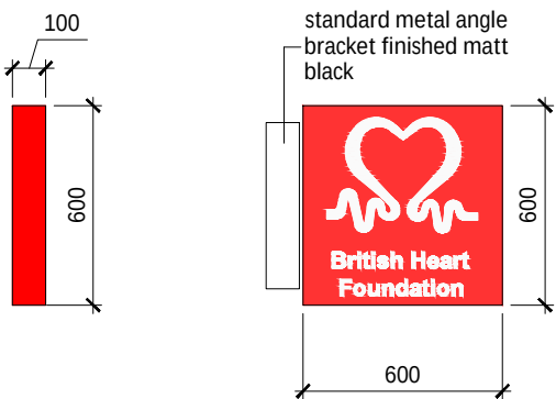
Sign 2: Projector Sign Detail (Scale 1/25)
