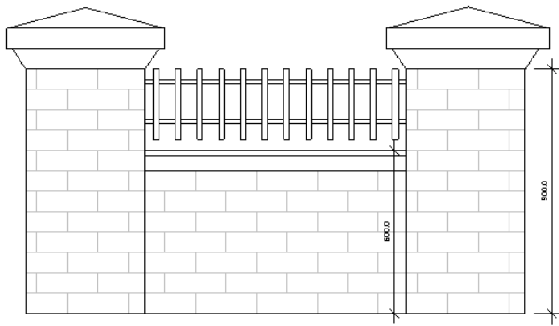
03 900mm high brick wall with fencing between brick piers (Front Boundary)
