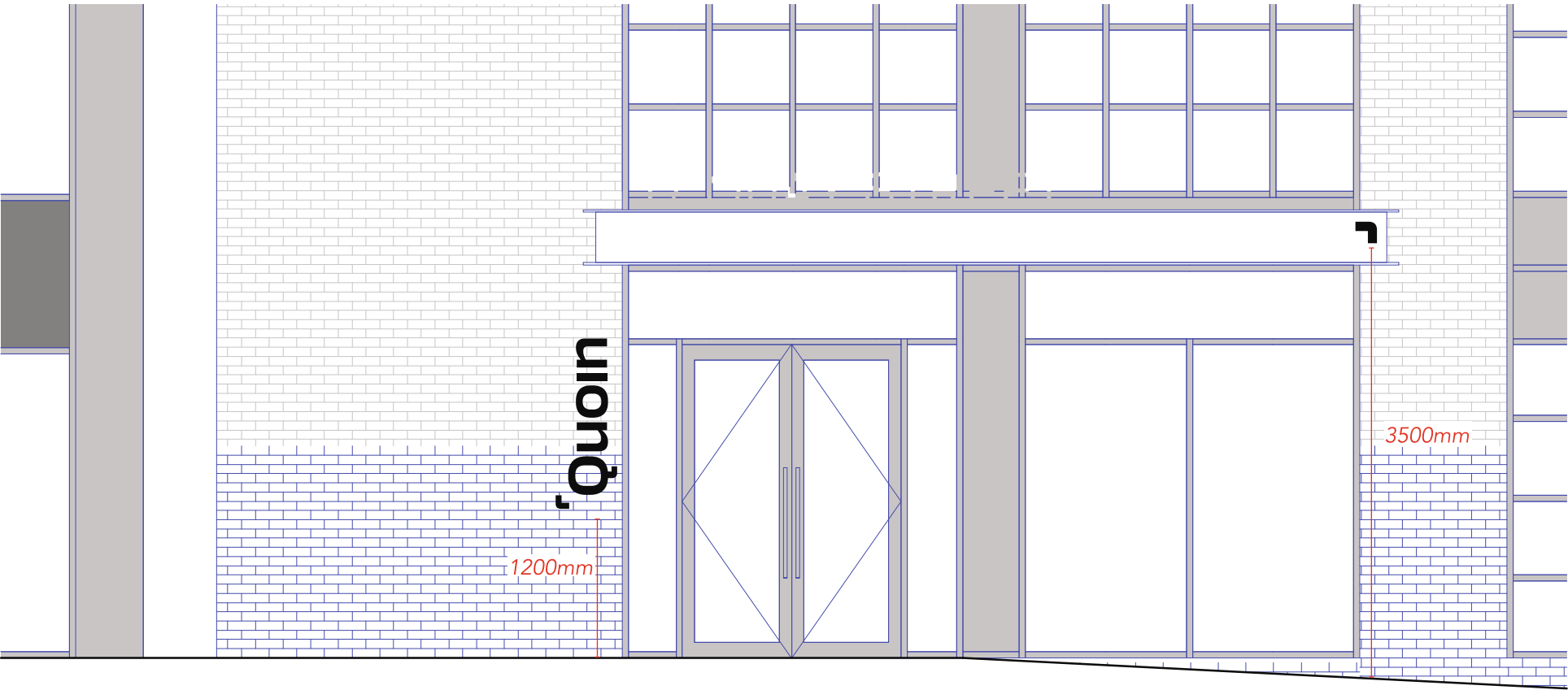
Indicative scale – 1:50
