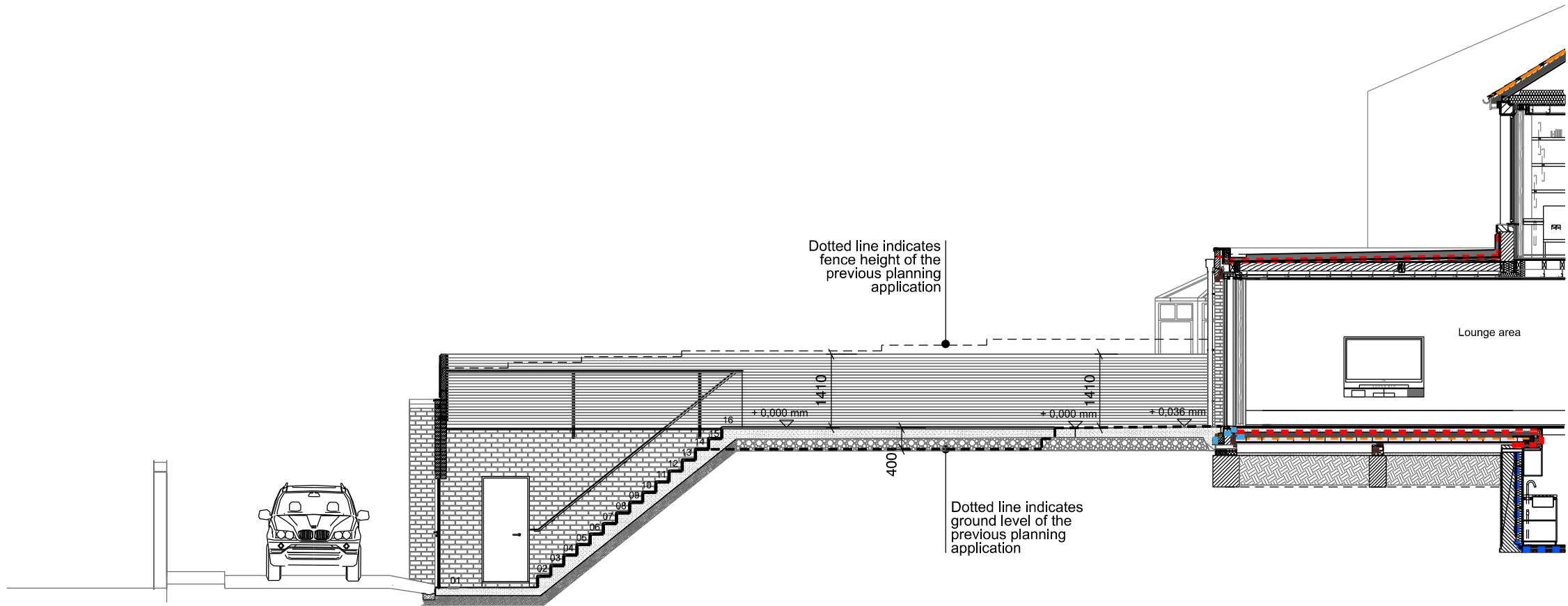
Proposed Section A
