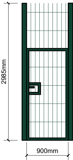
Elevation of Single Gate 1:50
