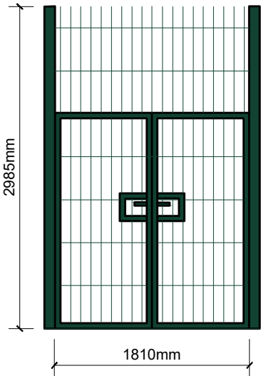
Elevation of Double Gate 1:50
