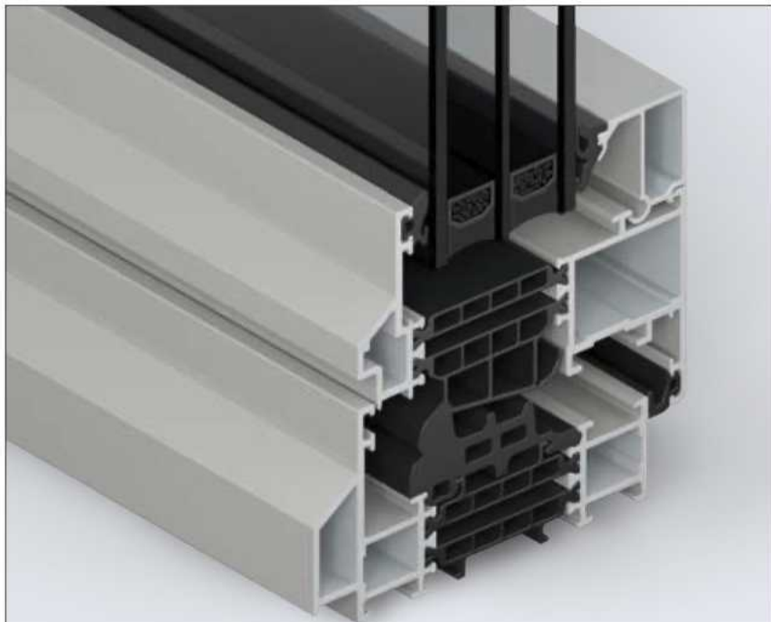
SOLEAL NEXT 75 Visible slope frame and slope vent
