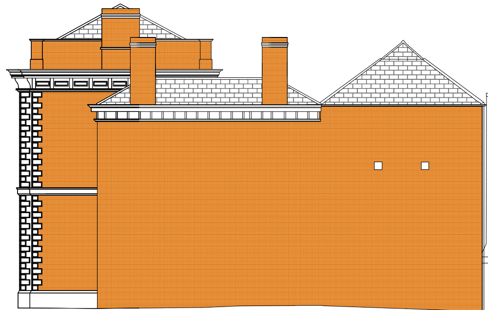
Existing Partial Side Elevation Scale - 1:200@A3
