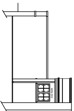
Orangery Courtyard Elevation (Easterly)
