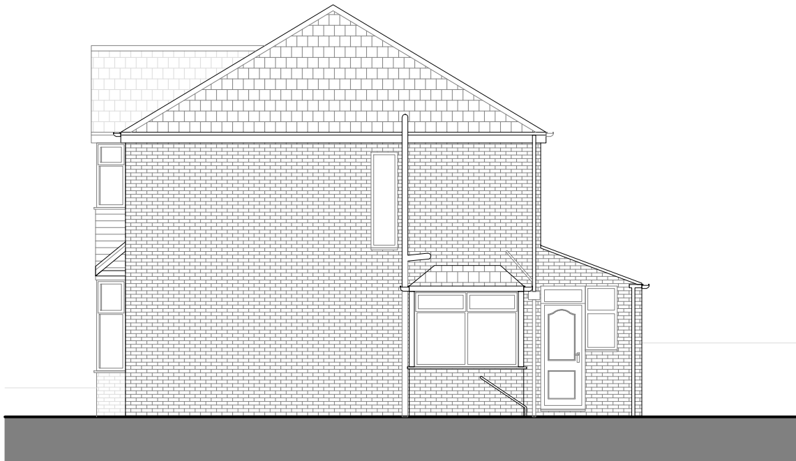
EXISTING REAR ELEVATION 1:100 @ A3
