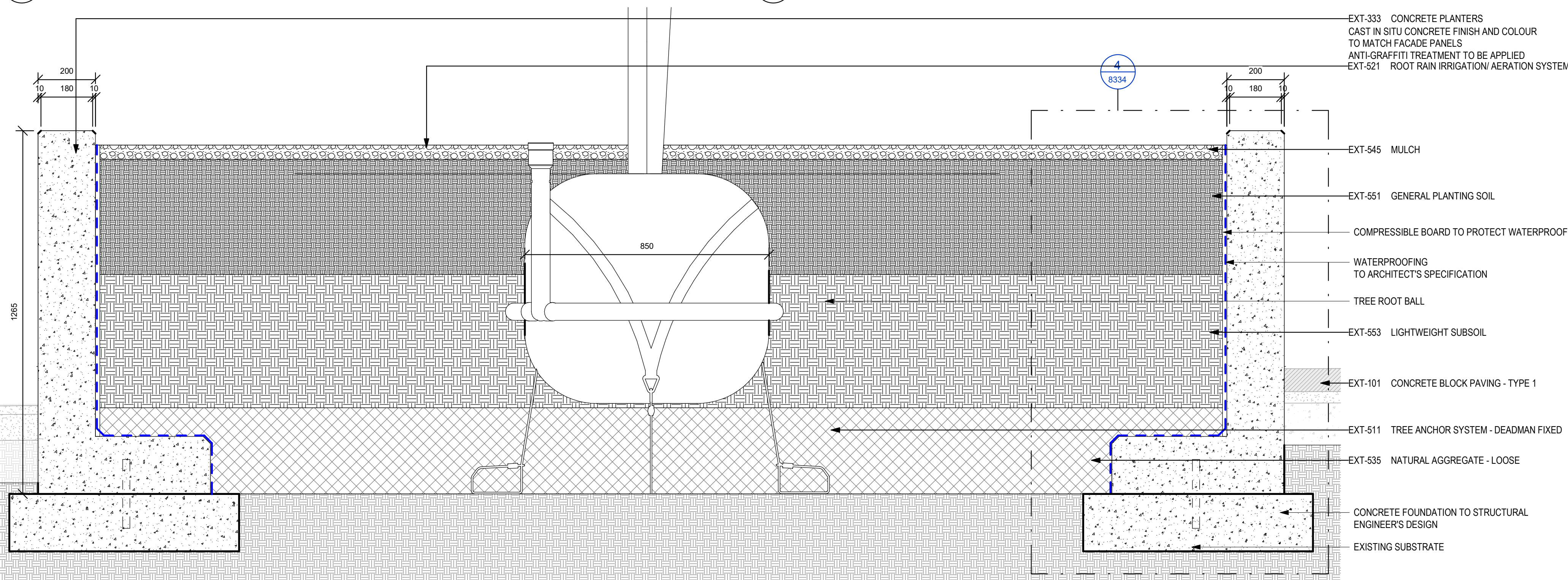
3 CAST IN SITU CONCRETE PLANTER P15 & P16 SECTION
