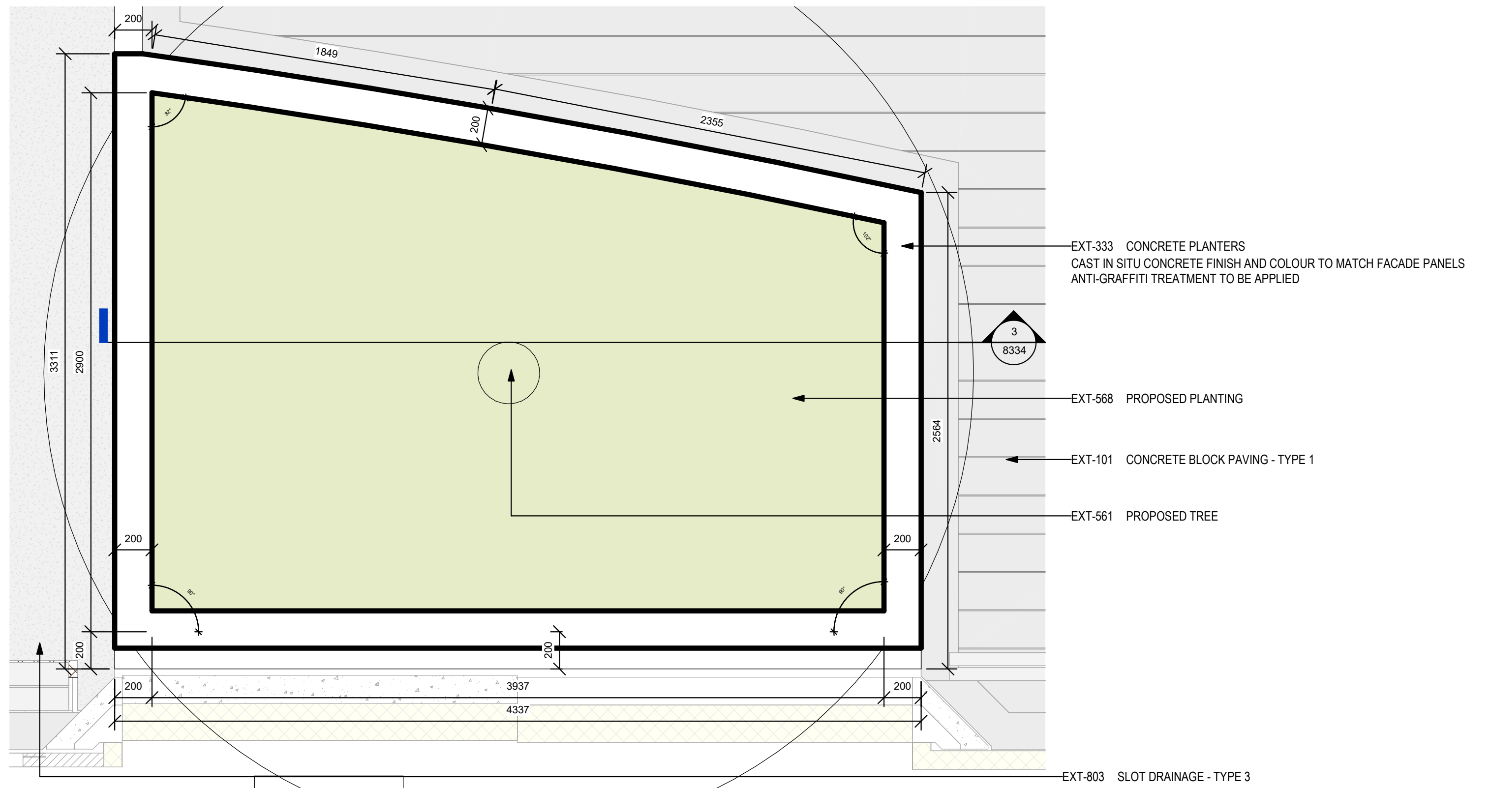
1 CAST IN SITU CONCRETE PLANTER P15 PLAN
