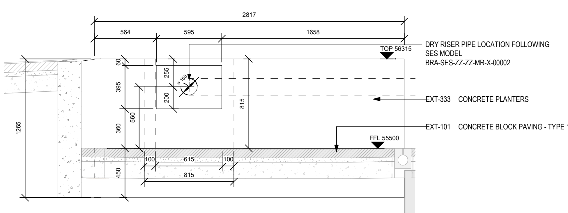
5 PLANTER P16 ELEVATION - WEST
