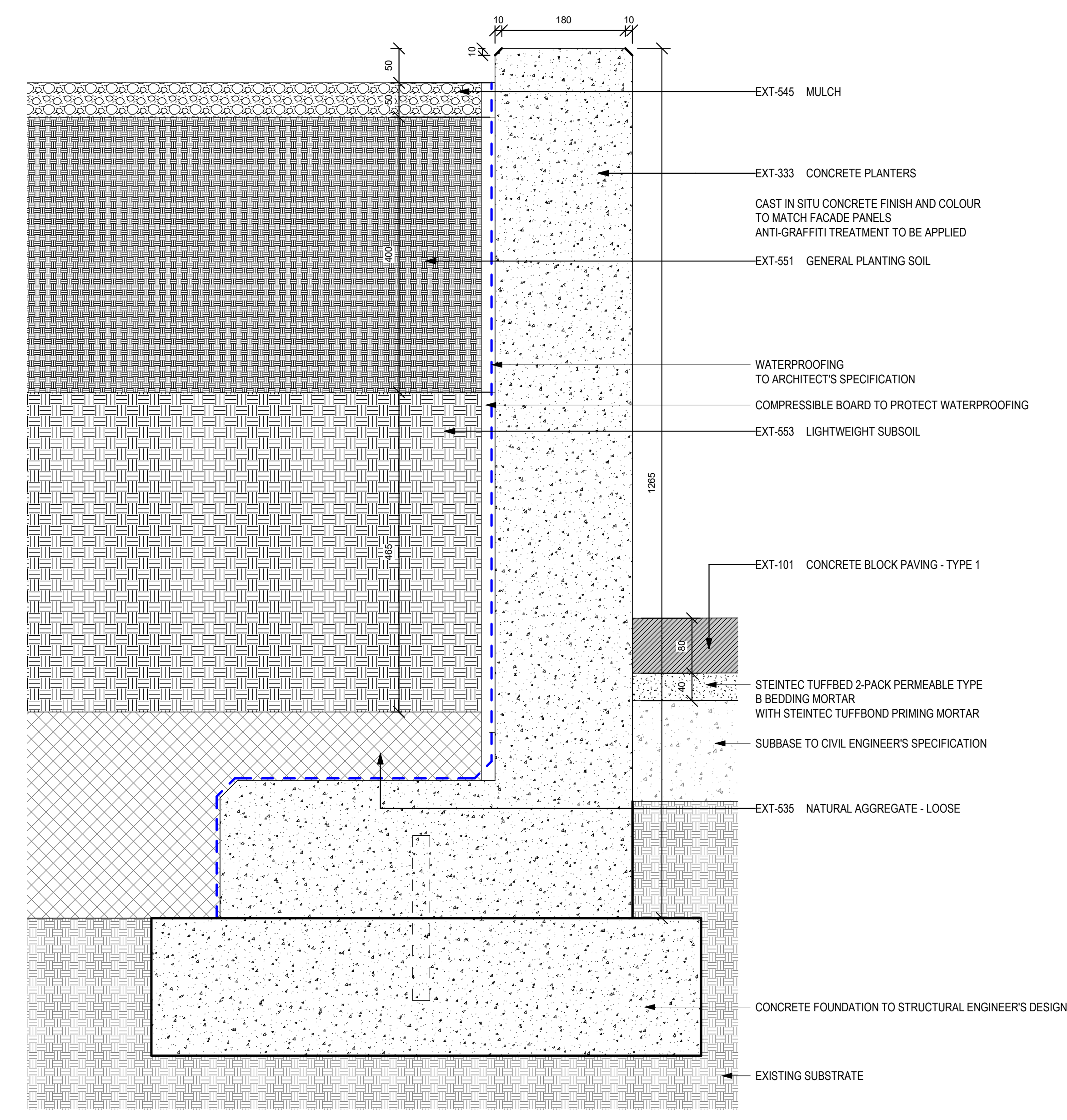
4 CAST IN SITU CONCRETE PLANTER P15 & P16 DETAIL
