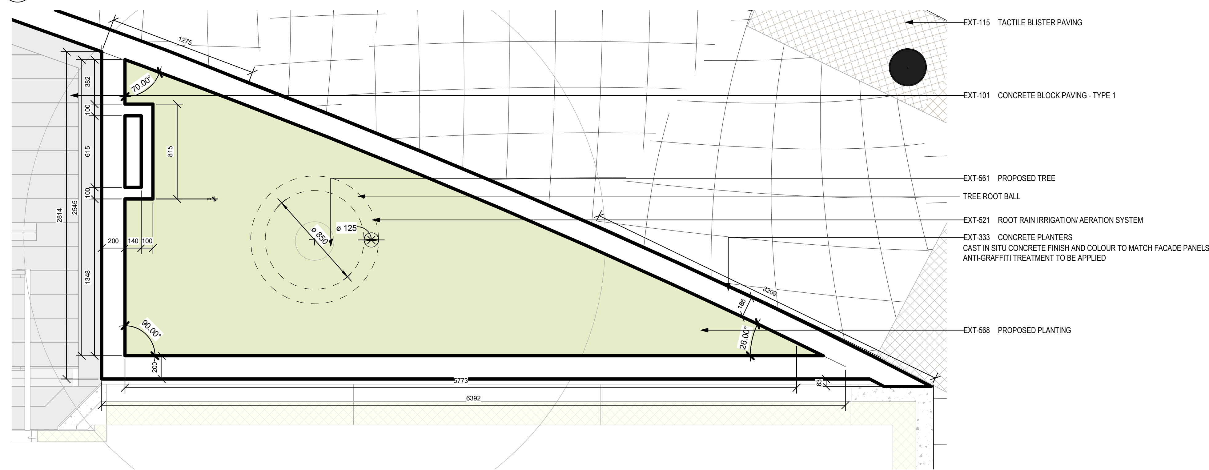
2 CAST IN SITU CONCRETE PLANTER P16 PLAN
