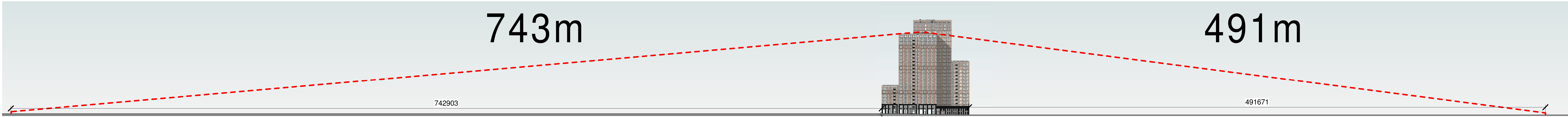
1 GA Elevation - Longacre St Level 22 plant sightlines 1 : 1250
