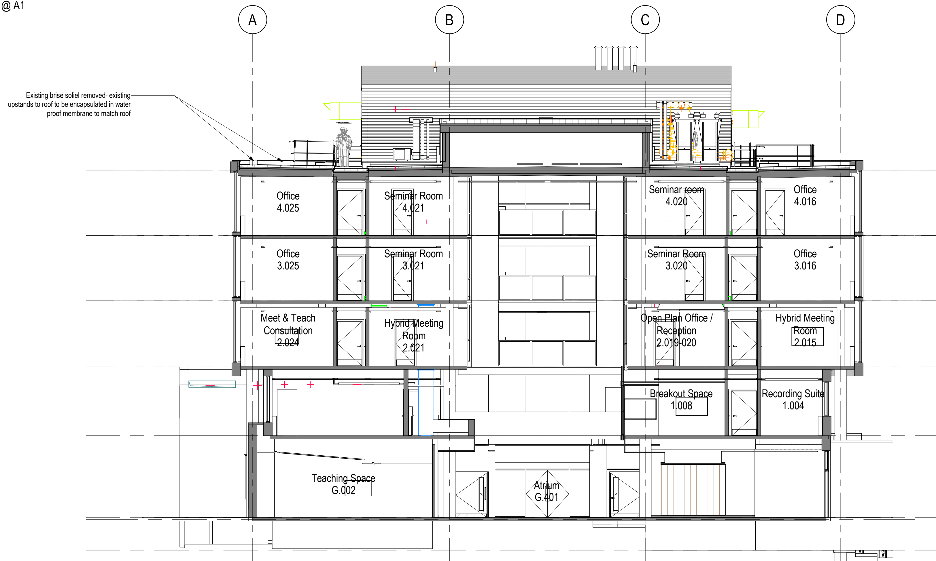
2 Proposed Section A-A Planning brise soleil 1 : 100 @ A1
