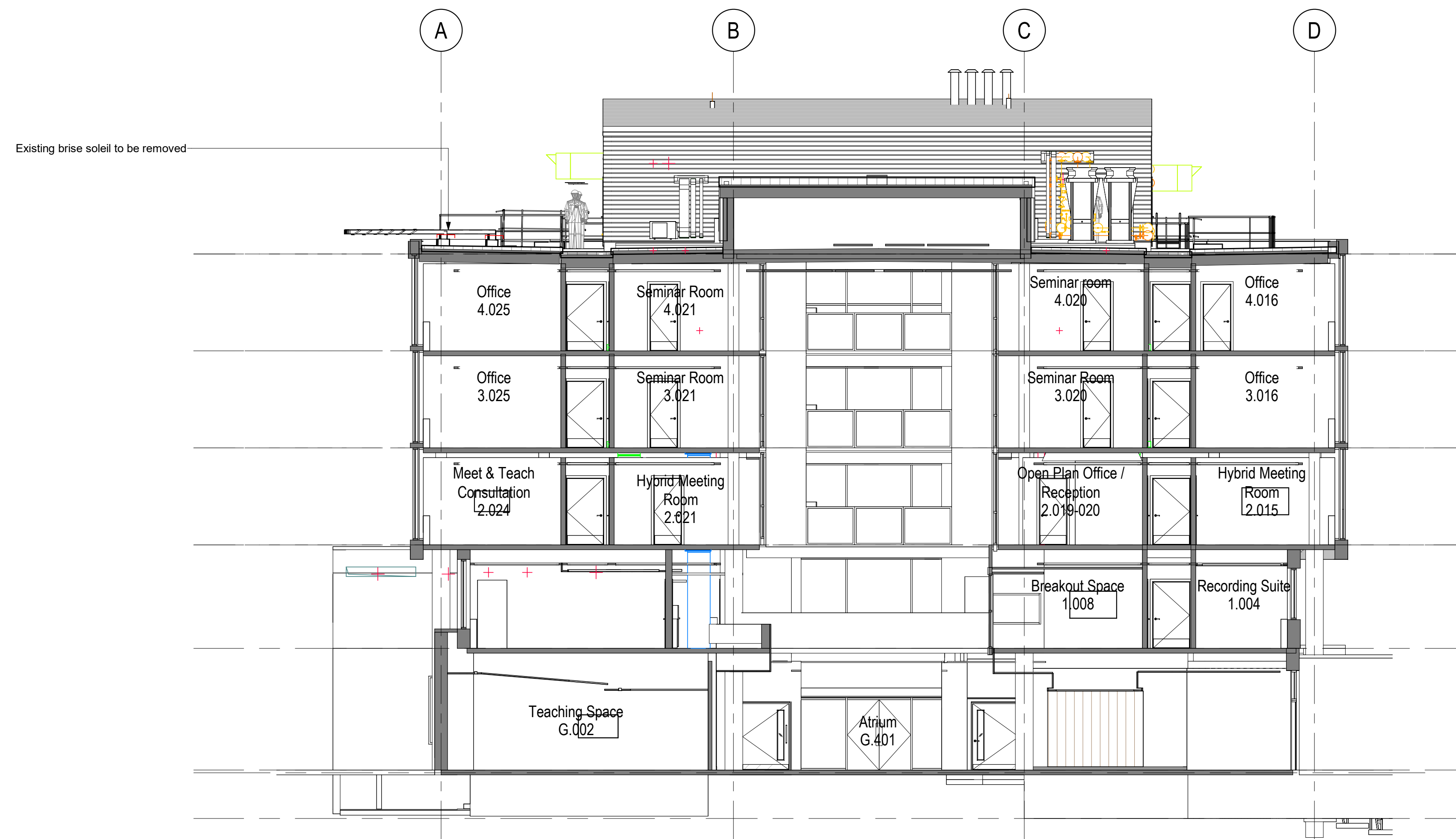
1 Existing Section A-A Planning brise soleil 1 : 100 @ A1
