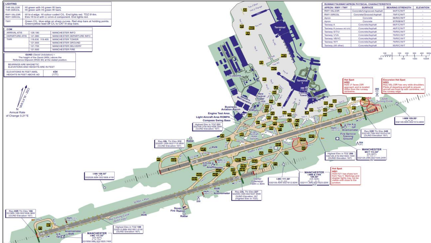
Figure 7 Aerodrome chart for Manchester Airport
