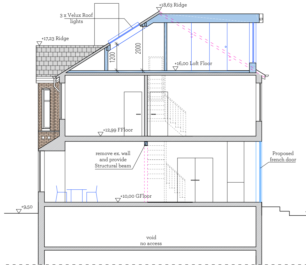
Proposed Section AA
