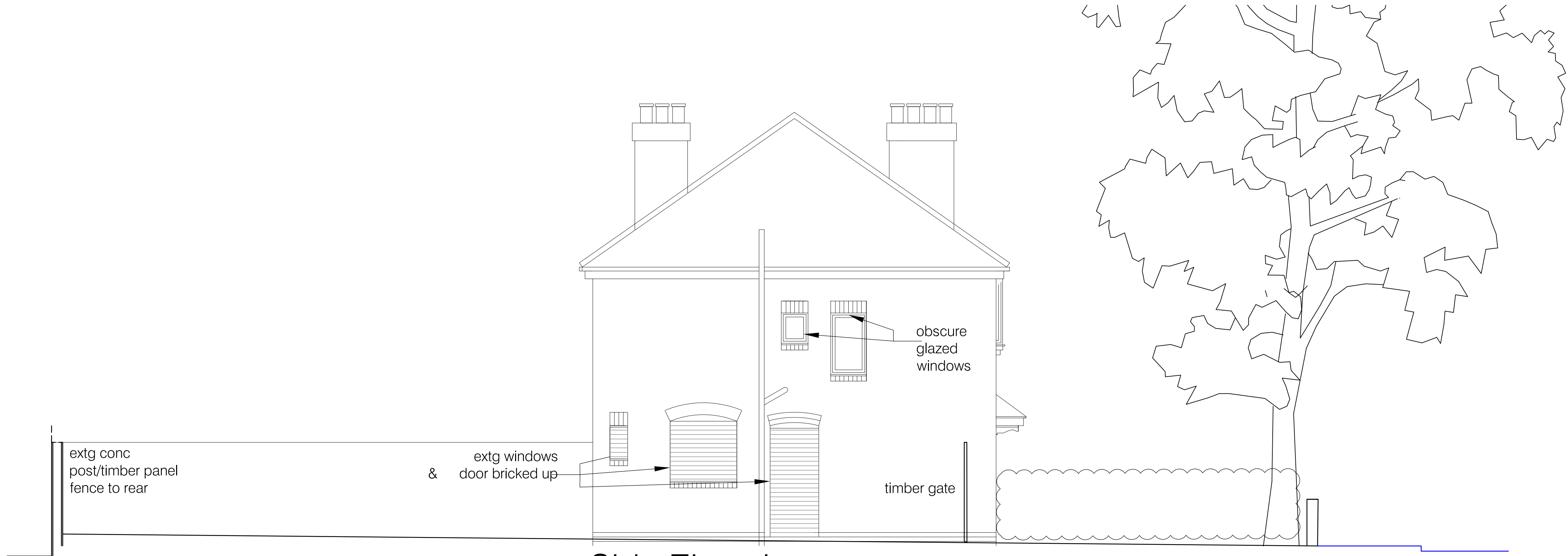
Side Elevation
