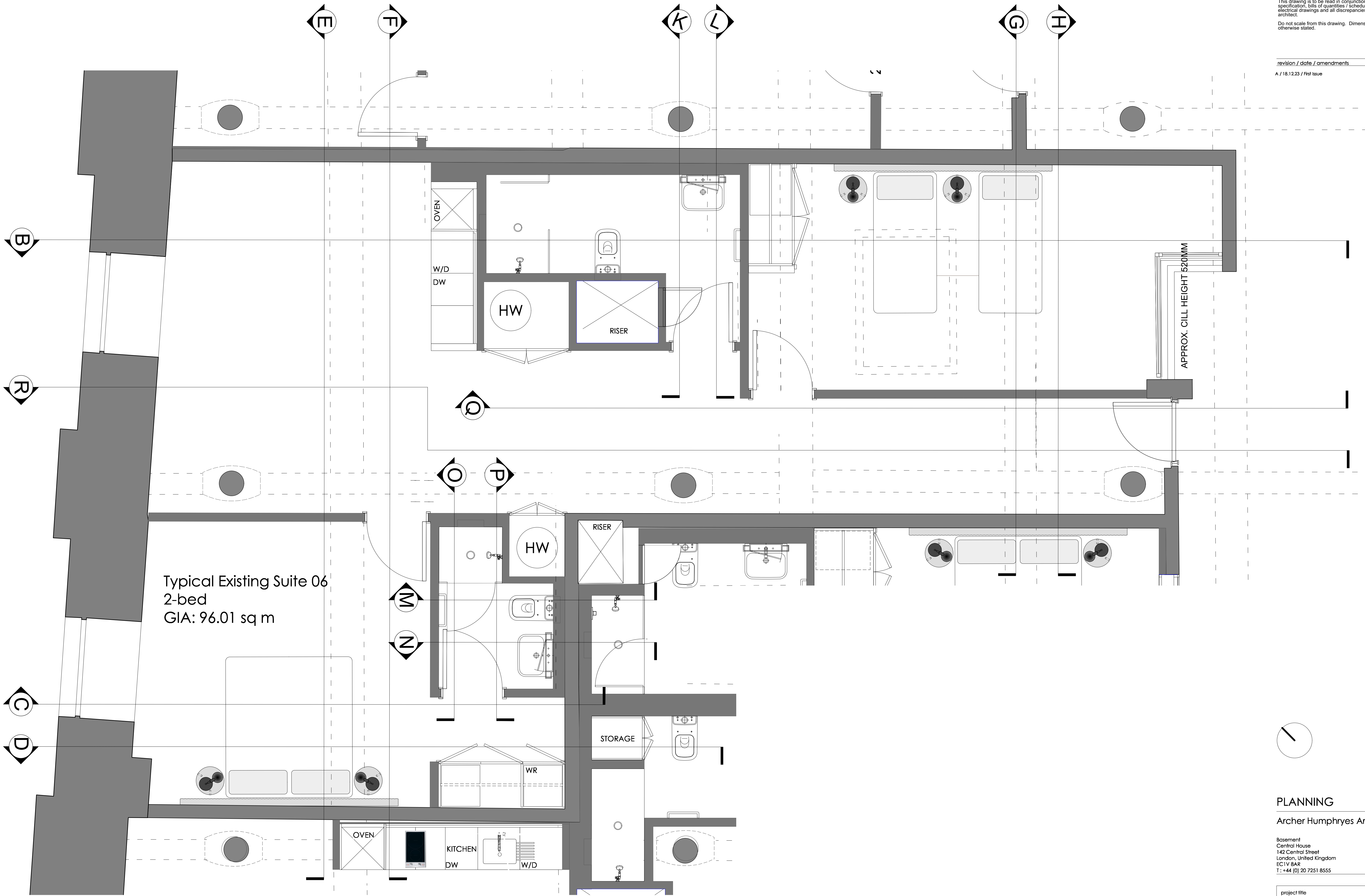
TYPICAL SUITE TYPE E - EXISTING PLAN
