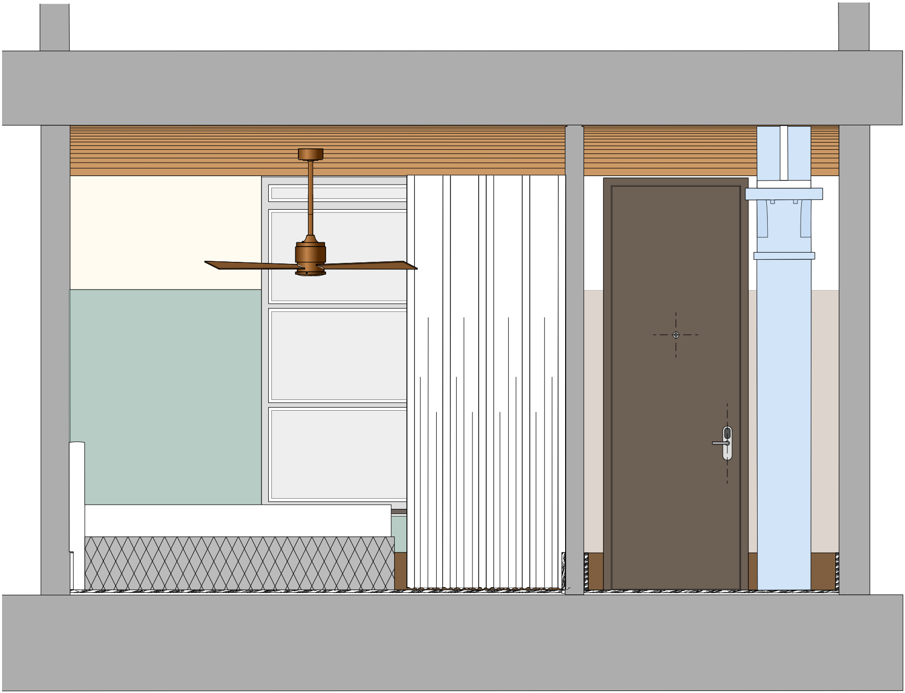
ELEVATION H
