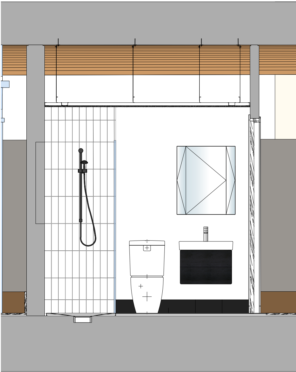
ELEVATION P
