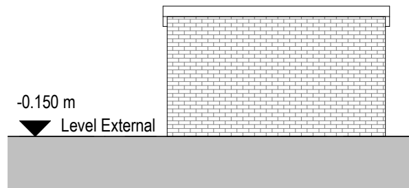
6 Rear Elevation - Outbuilding 1 : 100
