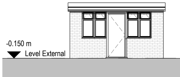
5 Front Elevation - Outbuilding 1 : 100
