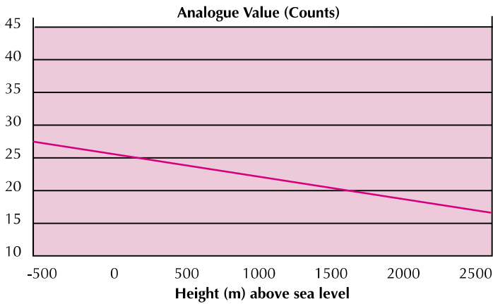
Fig.5 Typical pressure response - XP95 Ionisation Detector
