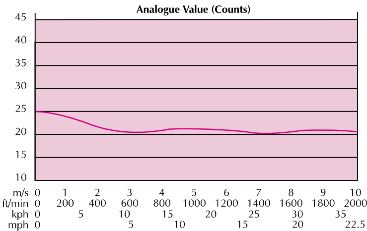
Fig.6 Typical wind speed response - XP95 Ionisation Smoke Detector
