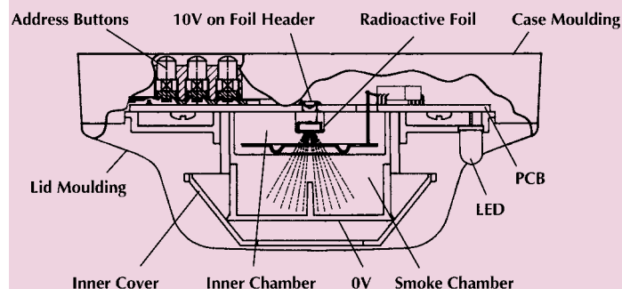
Fig.1 Sectional view - XP95 Ionisation Smoke Detector
