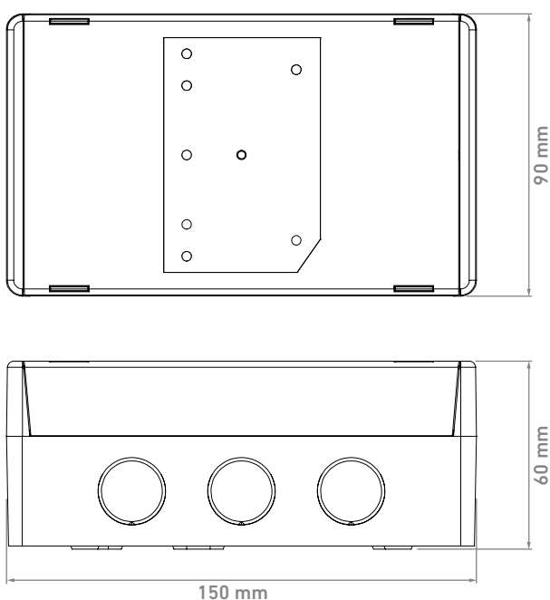
Figure 1: Intelligent Mains Switching Input/Output Unit dimensional drawing
