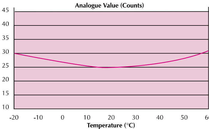
Fig.4 Typical temperature response - XP95 Ionisation Detector
