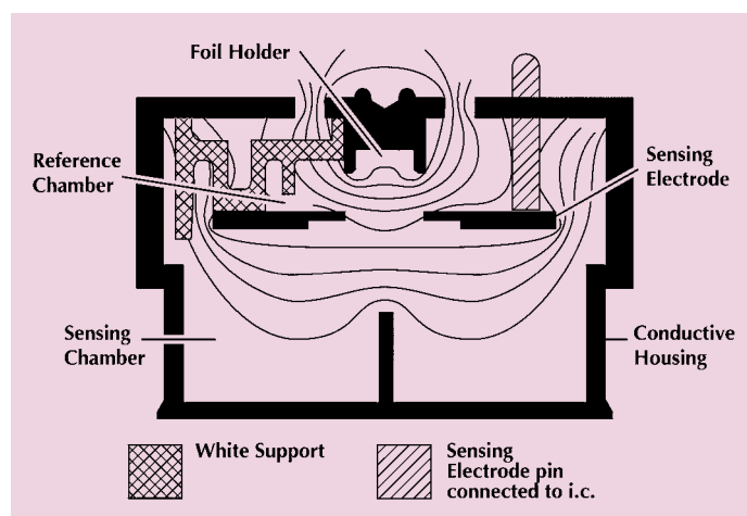
Fig.2 Diagram showing lines of equipotential for the XP95 Ionisation Smoke Monitor
