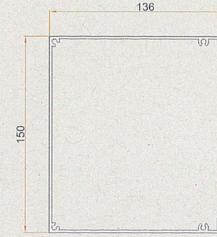
KF-0001 ANA ŞASE MOTOR BOX PROFILE
