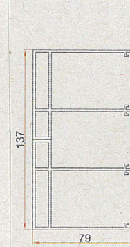
YAN KASA SIDE FRAME
