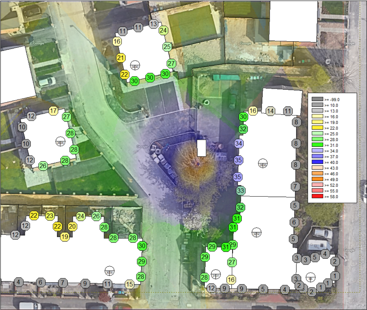
Figure 5.1: Calculated Sound Level (dBA) Based on Measured Data with ASHP Operational
