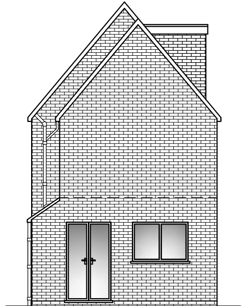
PROPOSED RIGHT SIDE ELEVATION
