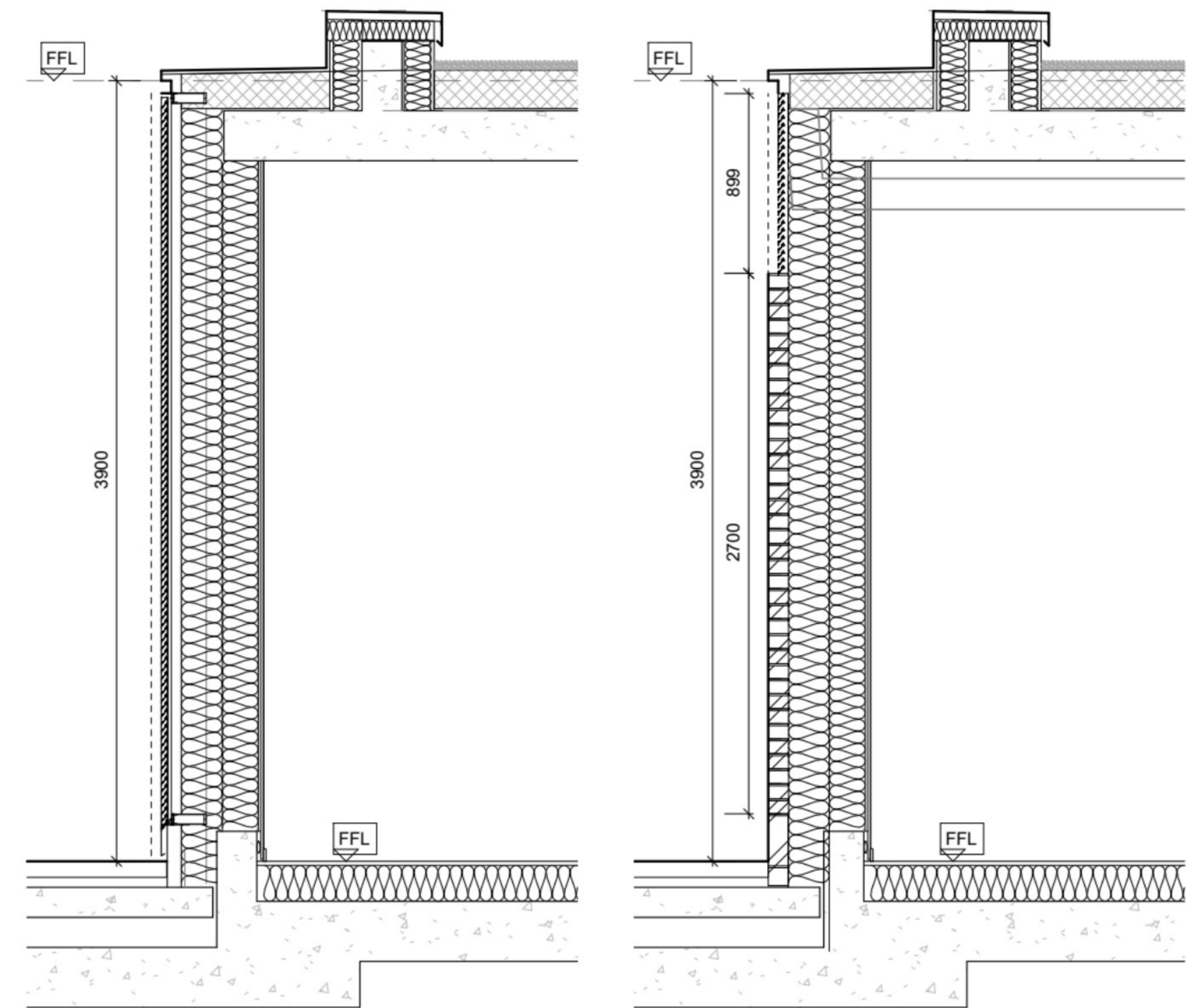
DETAIL SECTION AA
