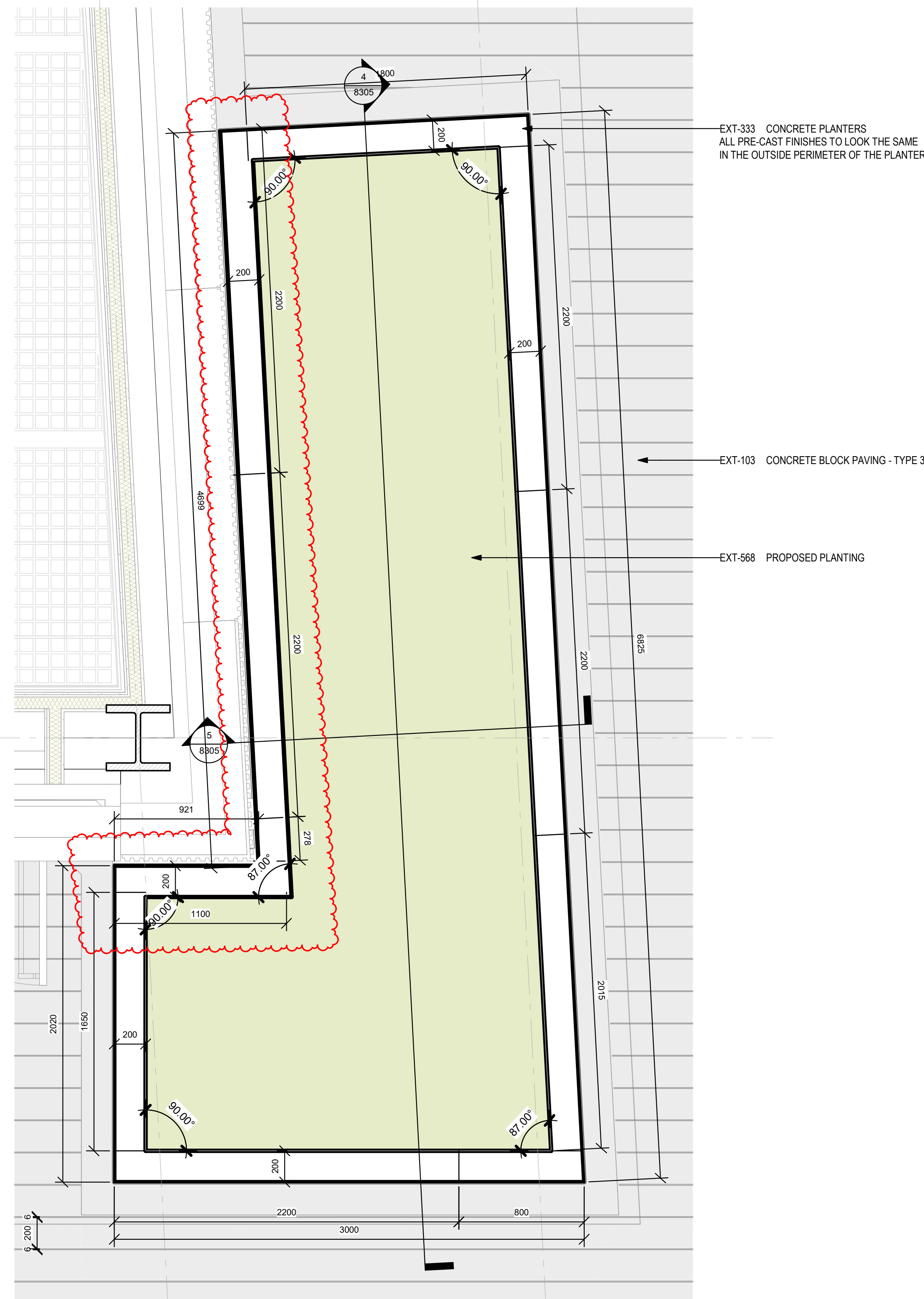
5 PRECAST CONCRETE PLANTER P8 PLAN
