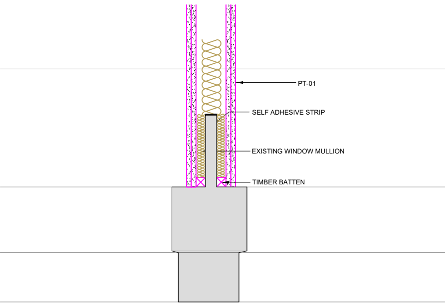
PARTITION TO WINDOW MULLION DETAIL 3
