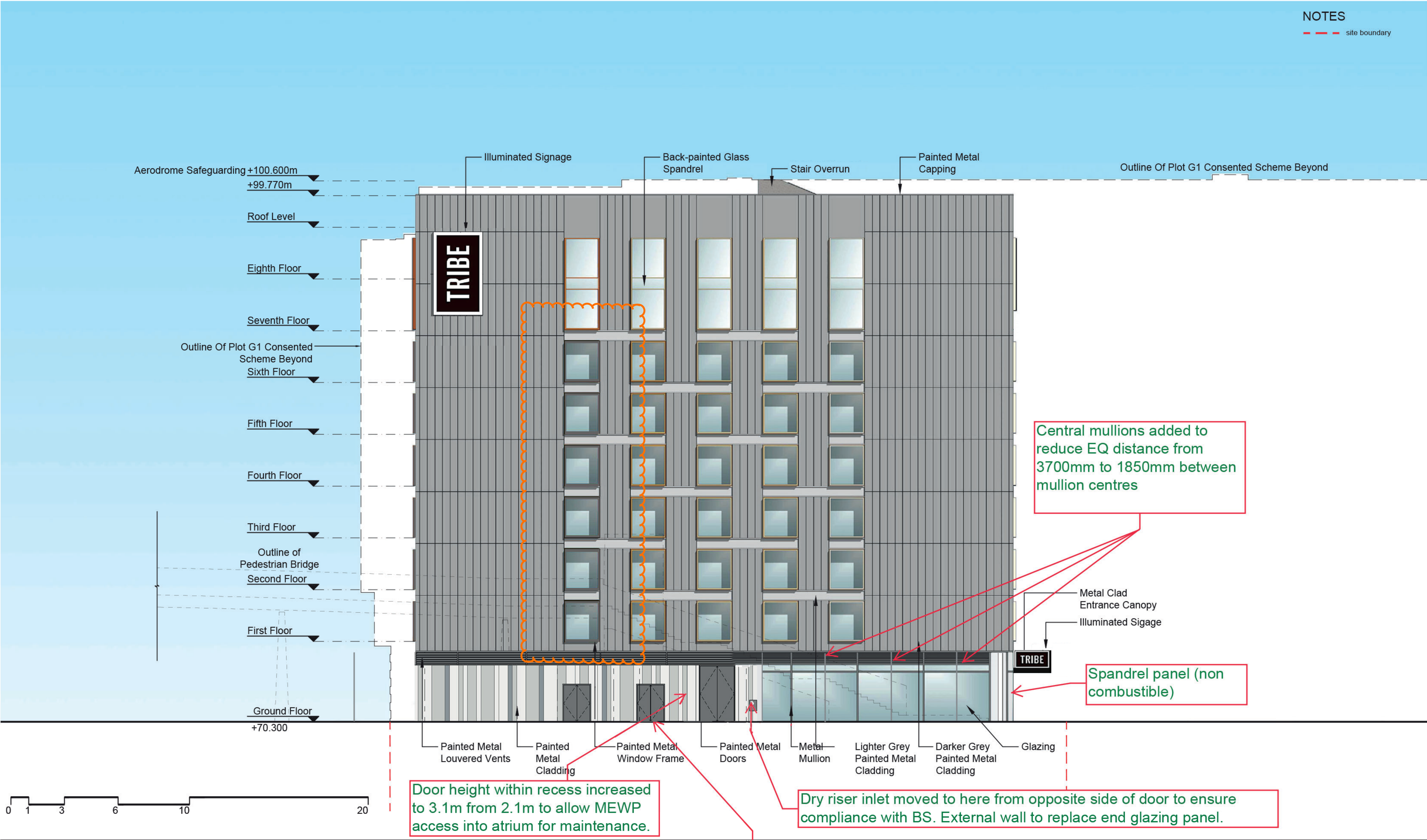
Proposed NW Elevation
