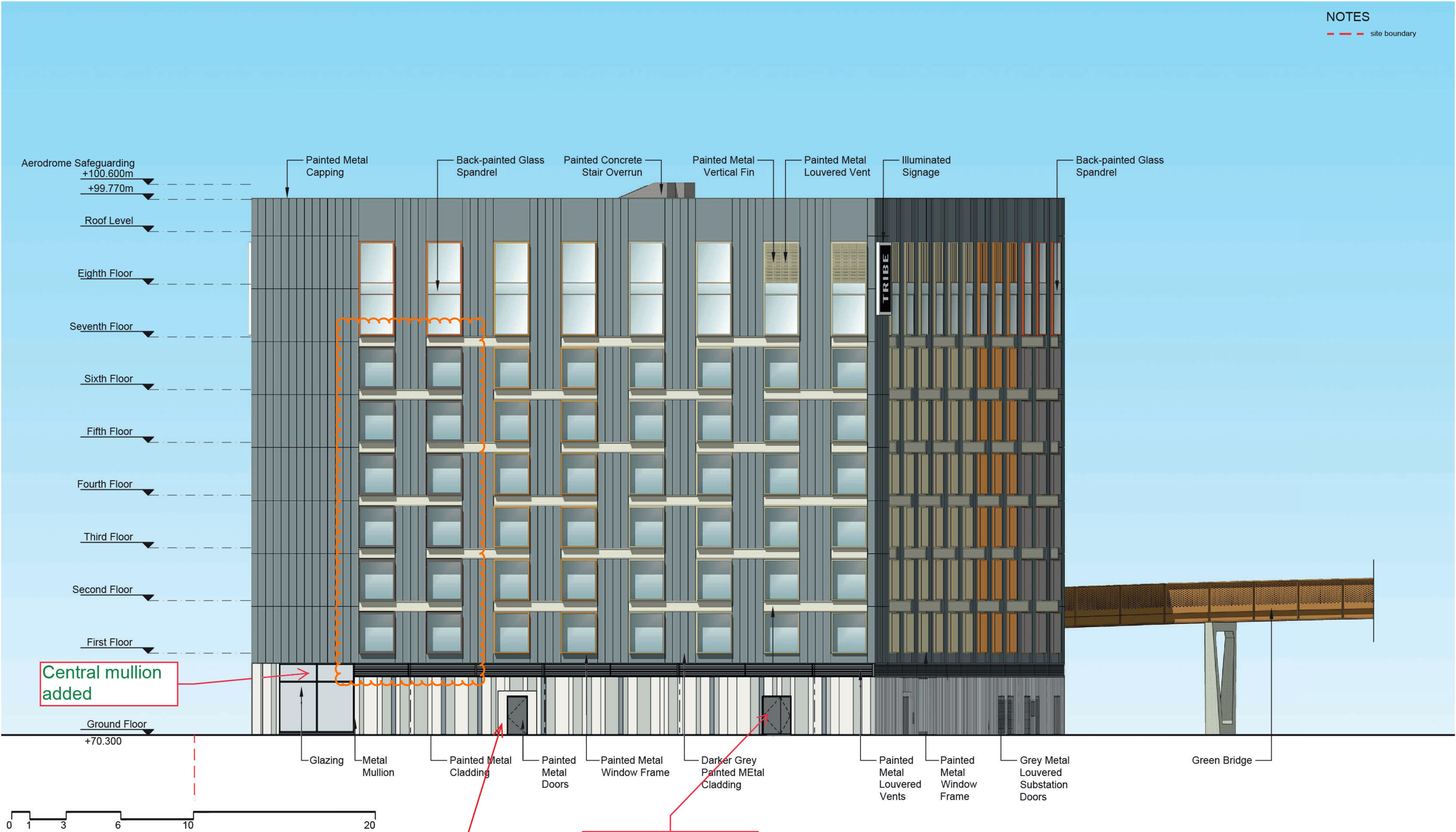
Proposed SE Elevation
