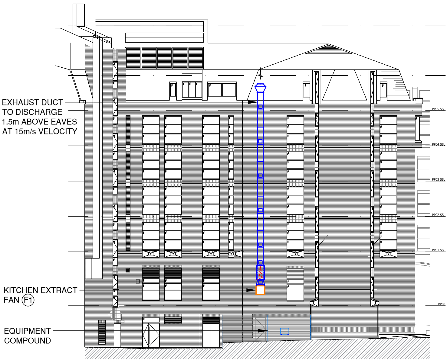
PROPOSED ELEVATION SCALE - 1:200
