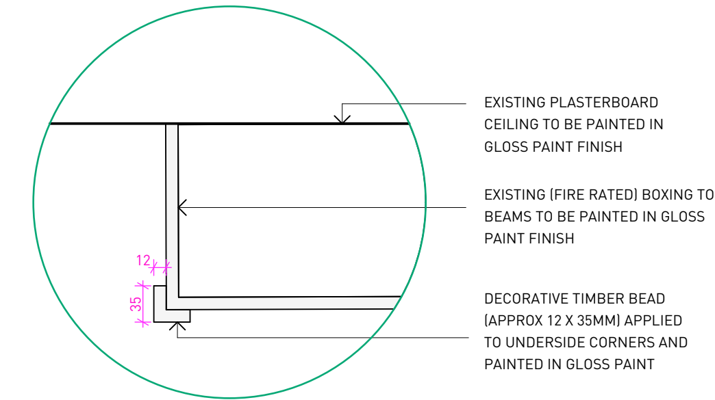
CF-09 (EXISTING FOH BEAMS) - TIMBER BEAD DETAIL
