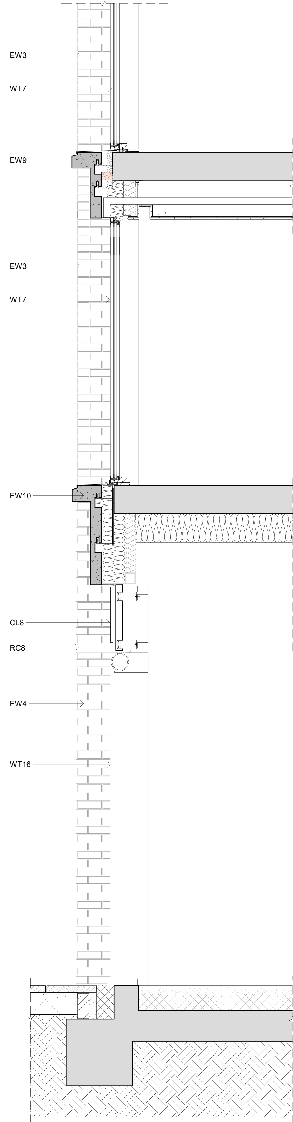
1-20 Detail Sections - Parking Bay_Planning 1 : 20
