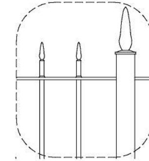
3 Railing Detail 1 : 10
