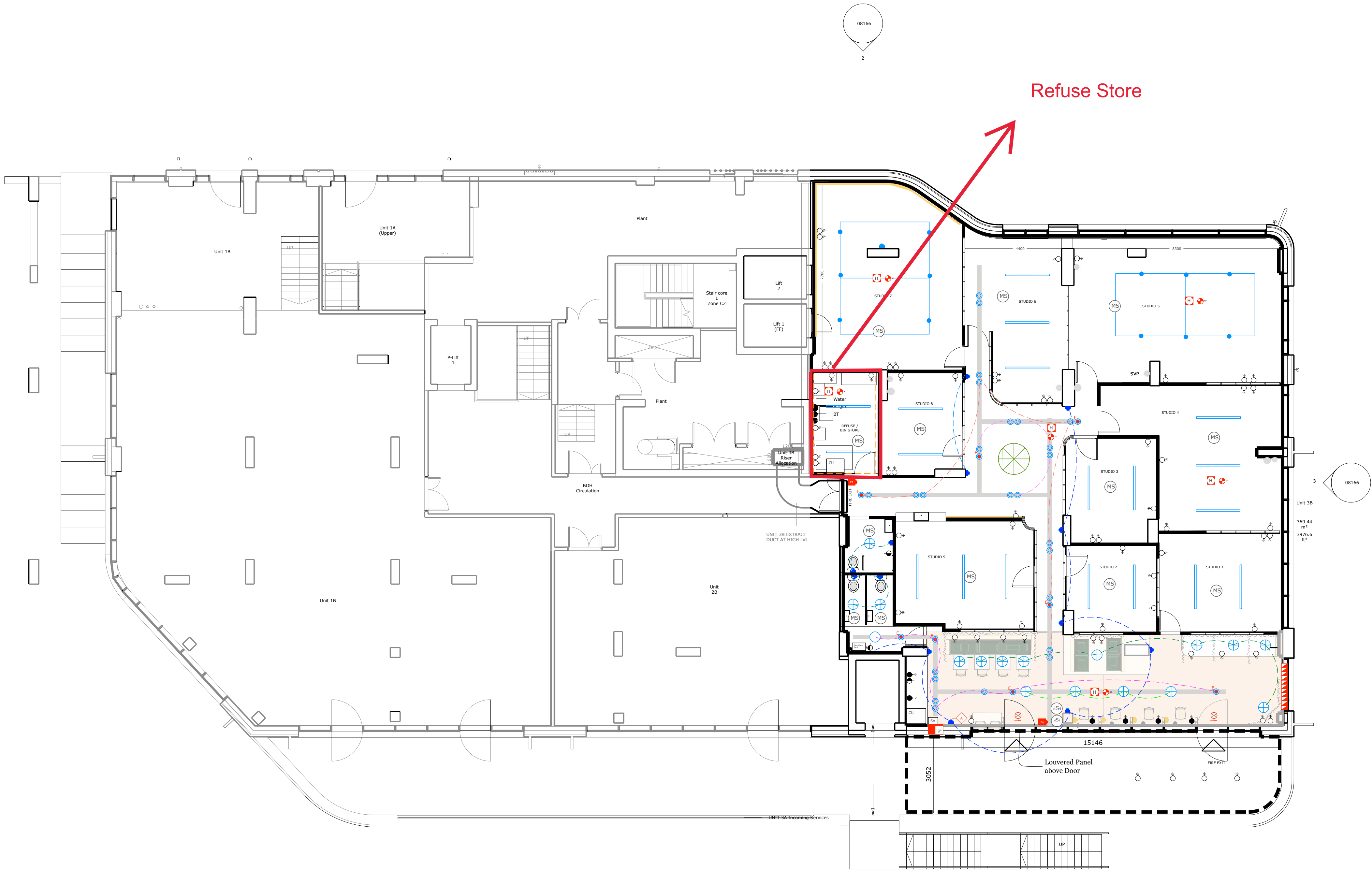
COMMERCIAL PLAN 1:100
