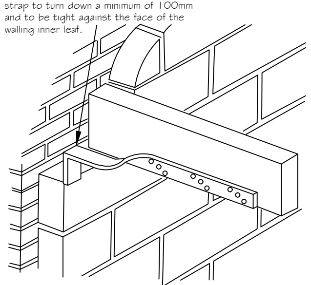
1:10 TYING OF TIMBER FLOOR BEARING ON TO WALL
