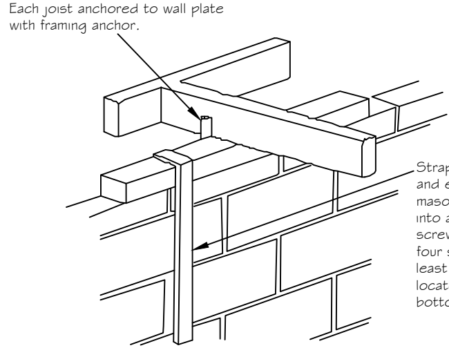
1:10 TYING OF TIMBER FLOOR BEARING ON TO WALL
