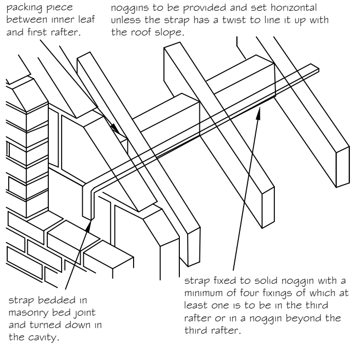
1:10 TYING OF PITCHED ROOFS TO GABLE WALLS
