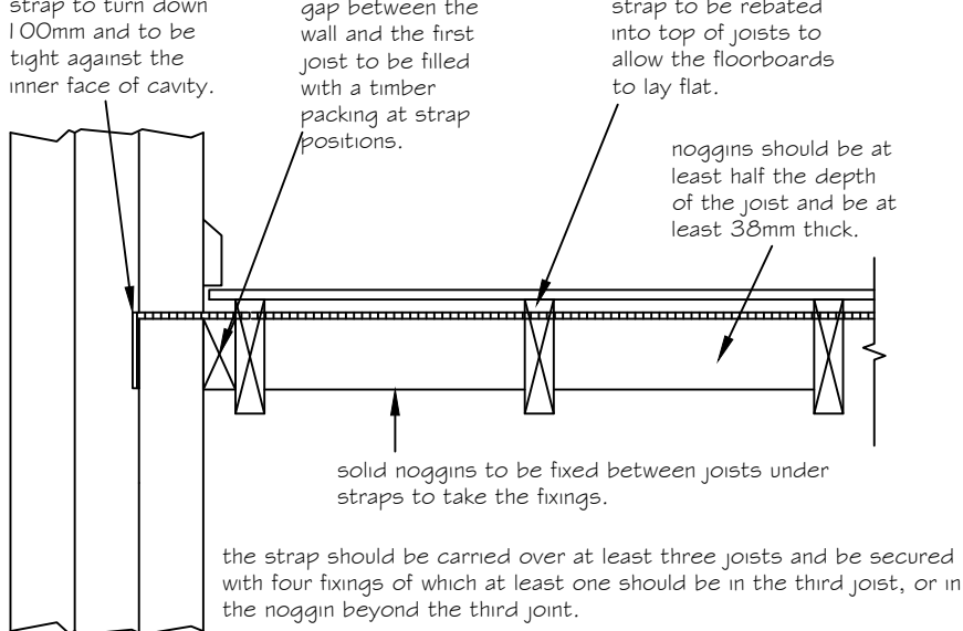
1:10 WALL RESTRAINT DETAIL WITH TIMBER FLOOR SPANNING PARALLEL
