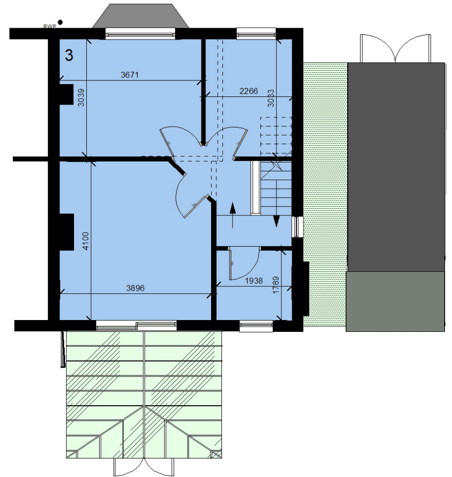
FIRST FLOOR - AS EXISTING
