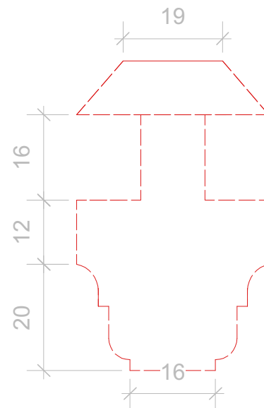
PROPOSED SECTION SIZES
