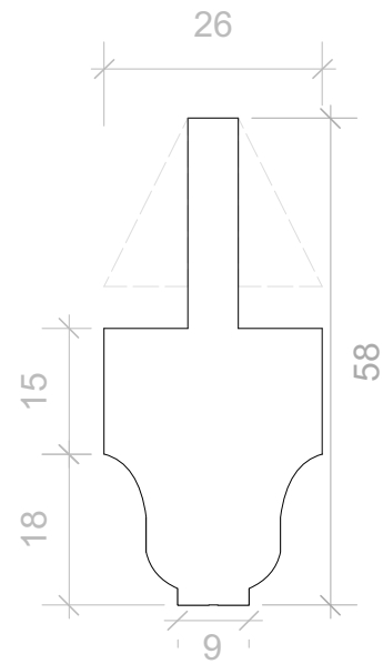
EXISTING SECTION SIZES
