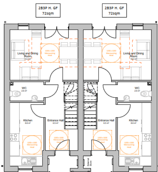
House Type - 2BH 72m² Ground Floor Plan
