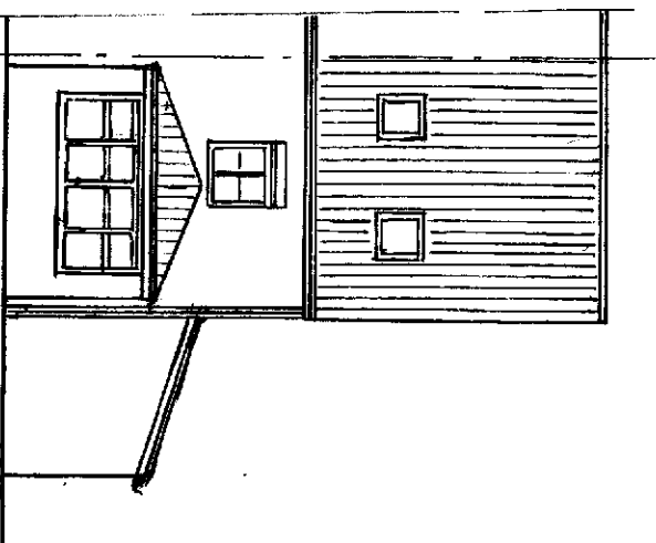
SIDE ELEVATION AS PROPOSED
