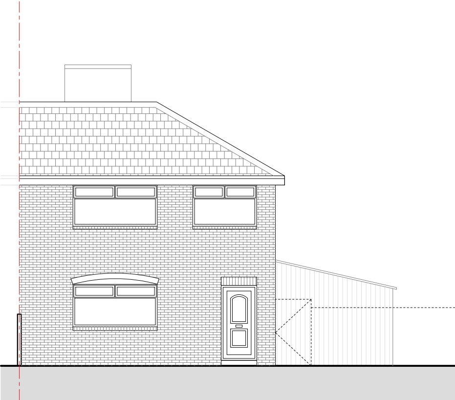
EXISTING FRONT ELEVATION 1:100 @ A3 0m 1m 3m 5m
