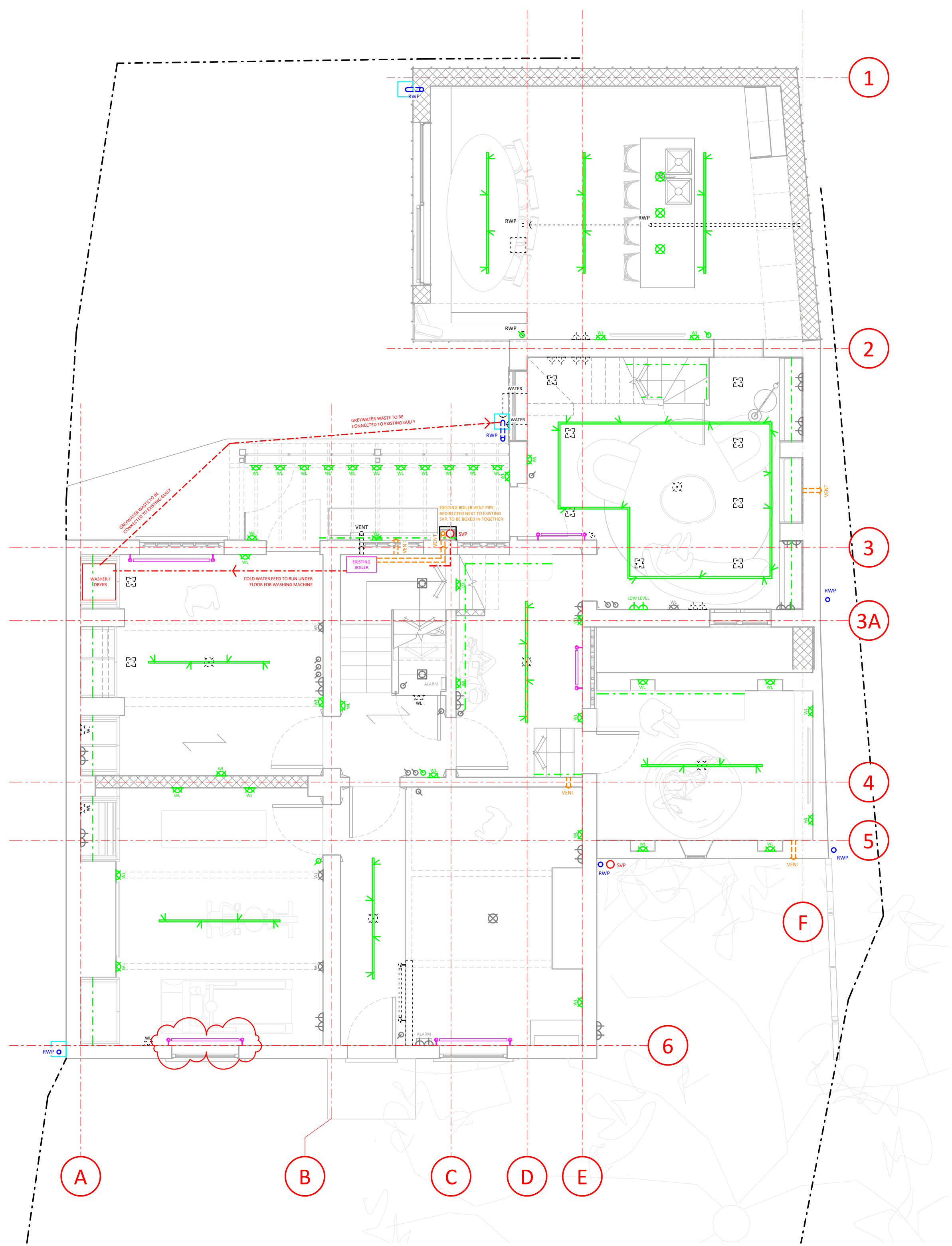
01 PROPOSED L0 M&E PLAN
