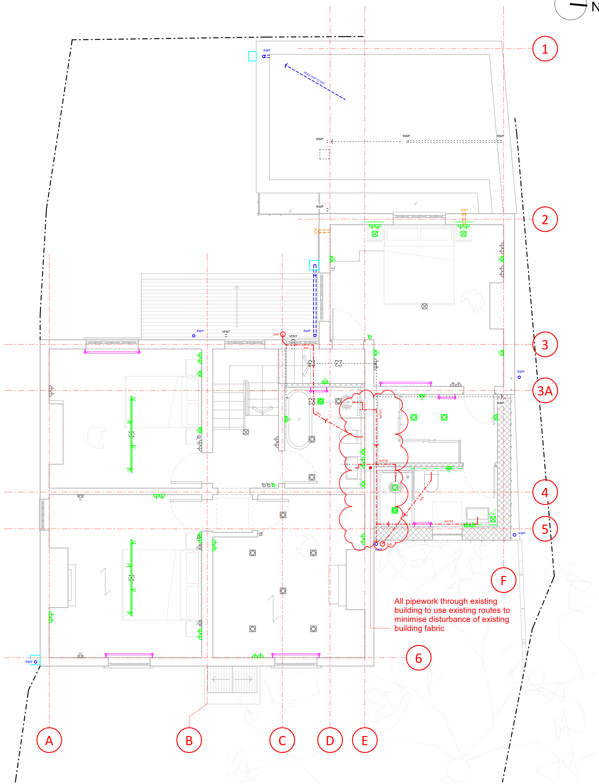
02 PROPOSED L1 M&E PLAN
