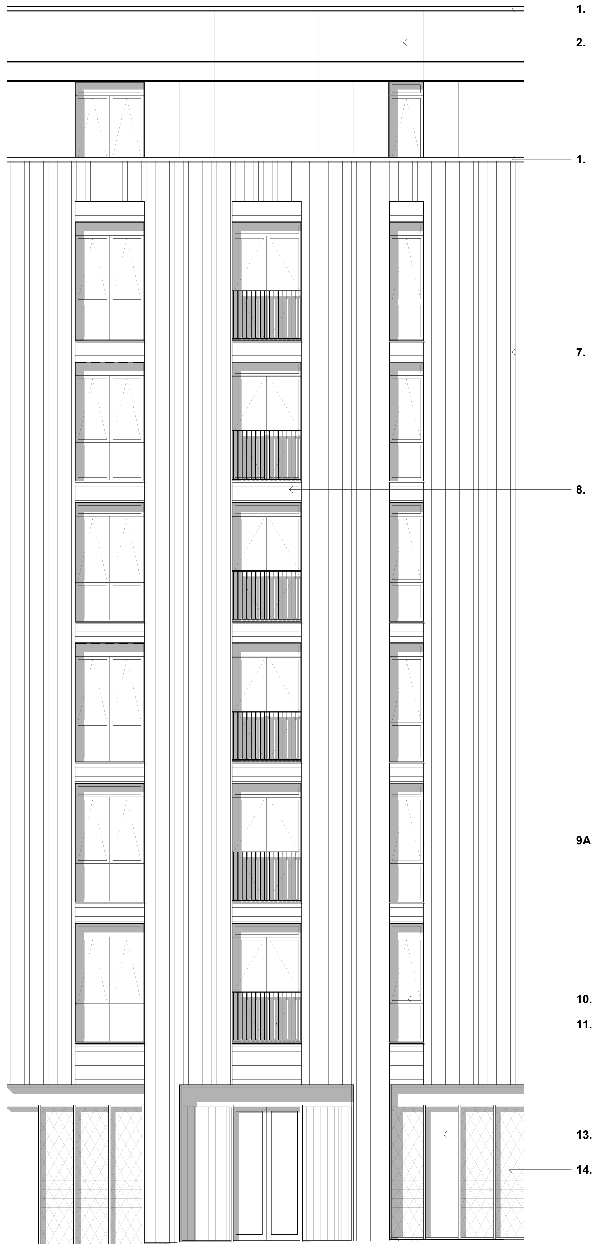
Bay Study 2 1 : 50
