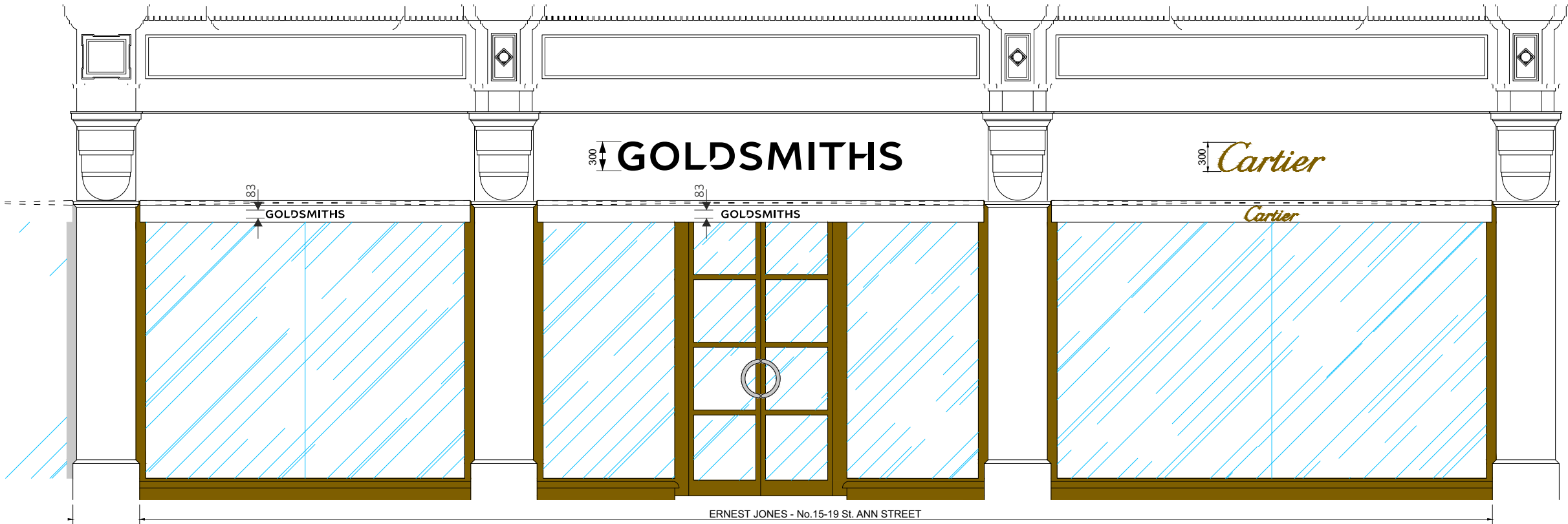
Proposed Elevation (Awning Closed) - Scale 1:50 @A3
