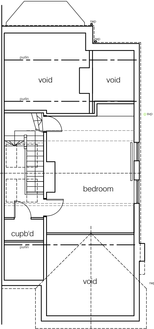
LOFT FLOOR PLAN AS EXISTING
