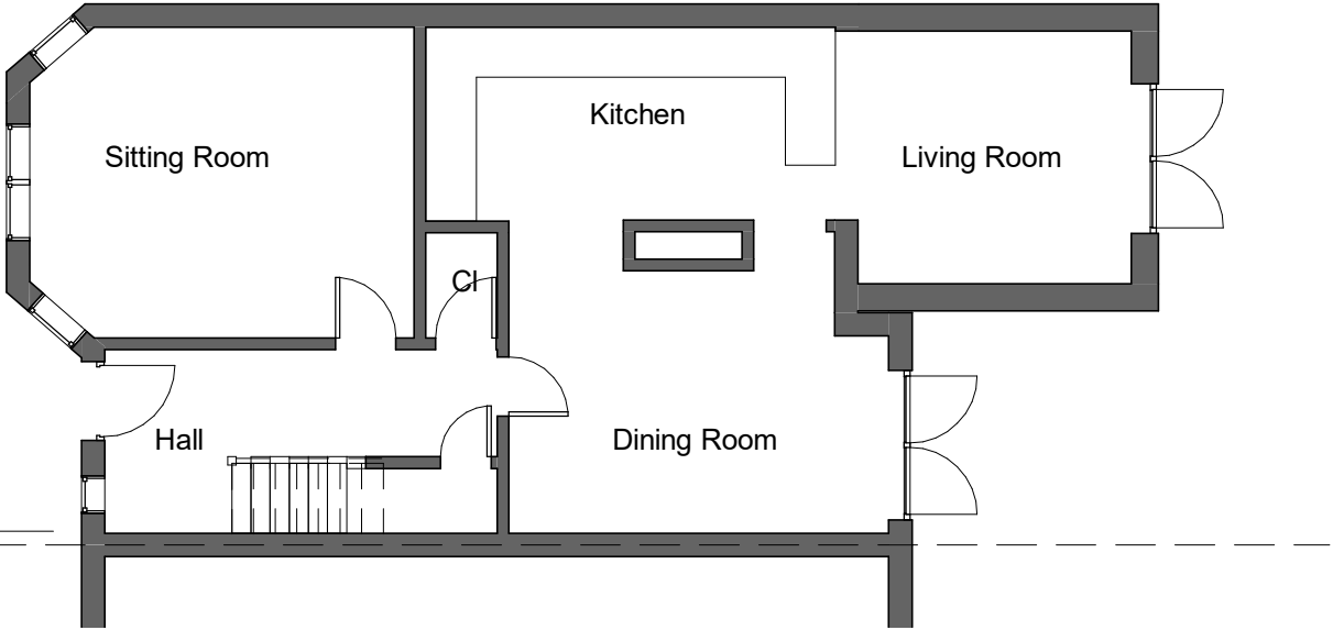
1 00 Ground Floor Existing 1 : 100
