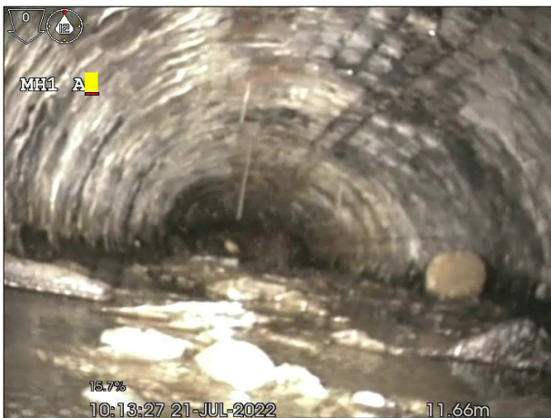
Photo: 11_11a, 00:00:00 11.66m, General Condition photograph
