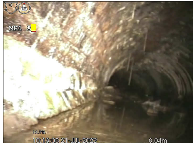
Photo: 1_10a, 00:00:00 8.3m, General Condition photograph
