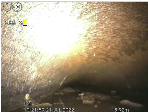
Photo: 24_8a, 00:00:00 8.92m, General Condition photograph
