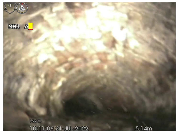
Photo: 1_7a, 00:00:00 5m, Debris silt, 40 % cross-sectional area loss, Changed
