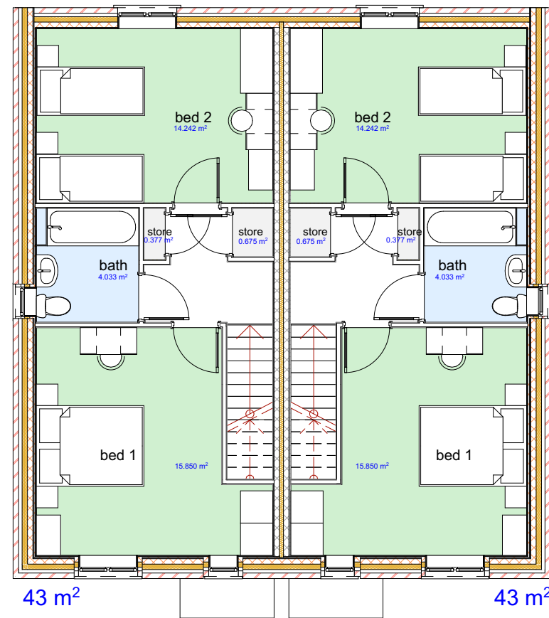
01-First Floor
