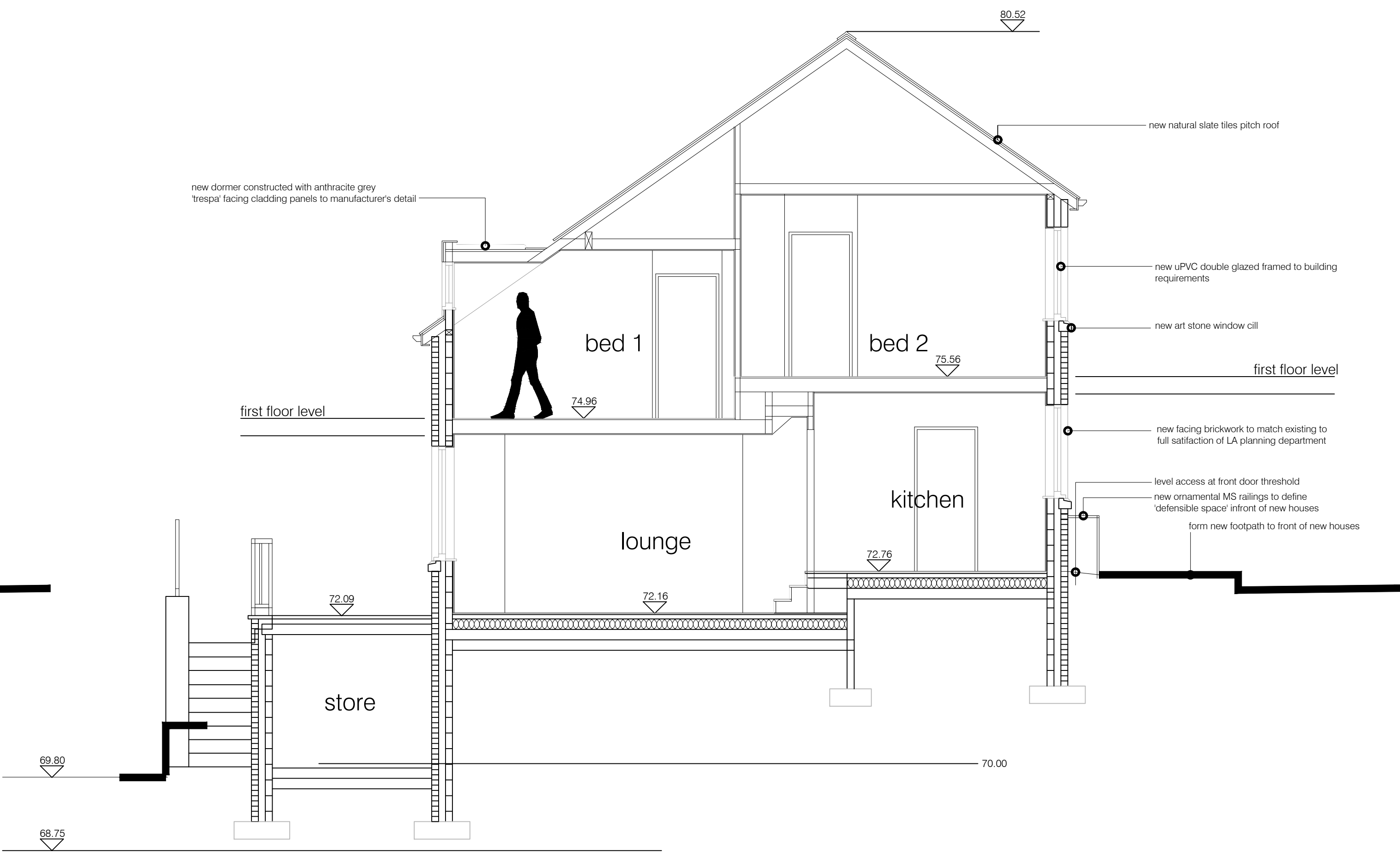
section Y-Y as proposed
