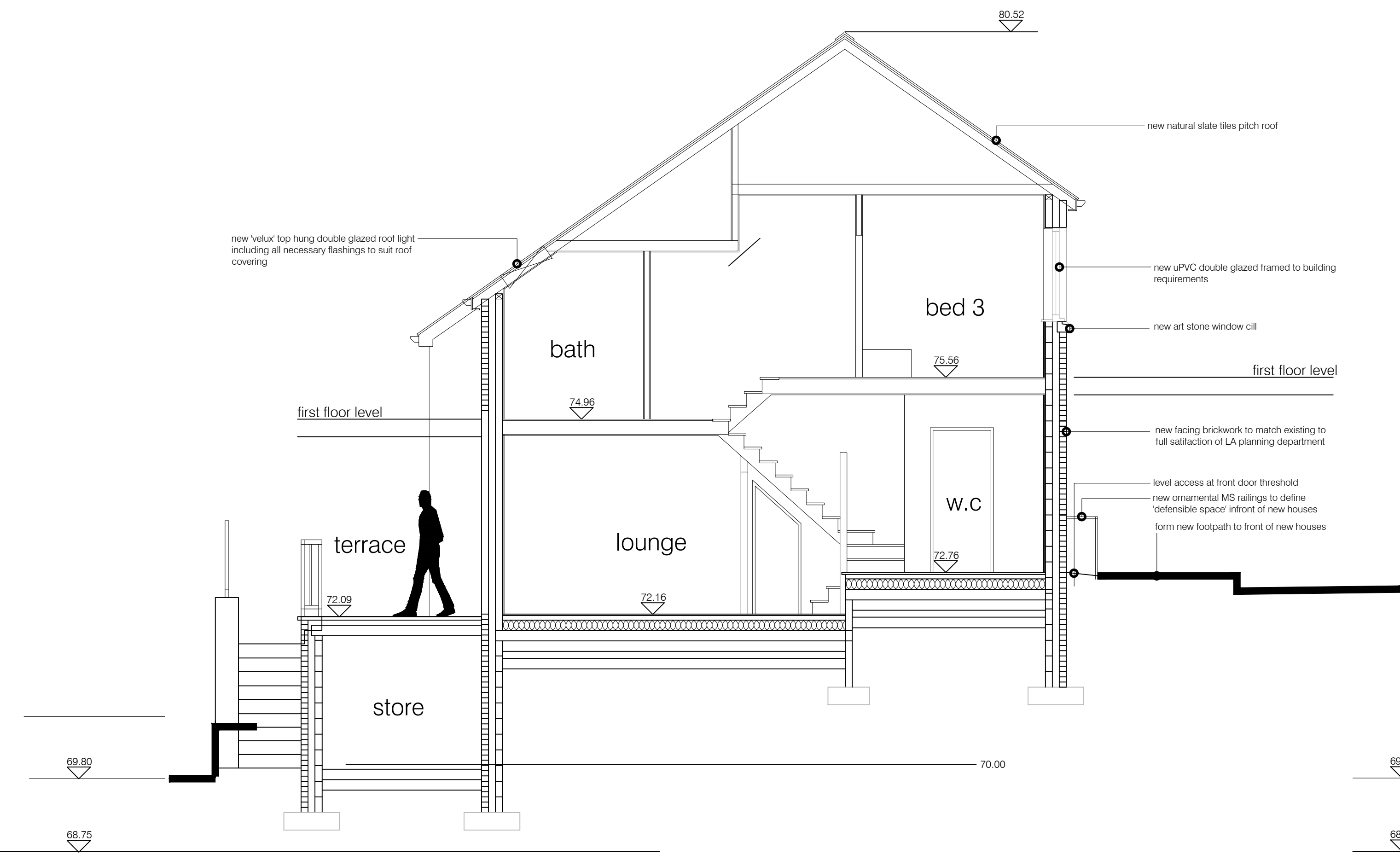
section X-X as proposed
