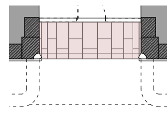
3 Localised Reflected Ceiling Plan Scale: 1:100
